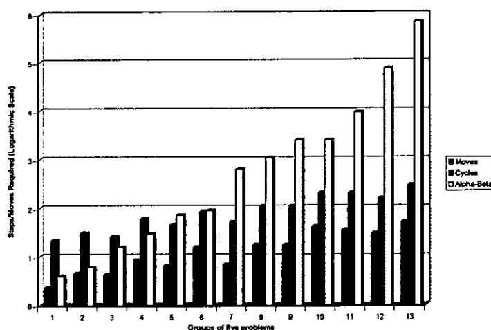
Fig. 8. This graph shows the number of moves and planning cycles taken by GoBI, plus the estimated \alpha-\beta search space size for the 63 correctly answered problems from test set I.
