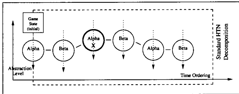
Fig. 4. Goal decomposition in “standard” HTN planning. The dashed arrows represent the decomposition of goals (eventually) into concrete actions.
