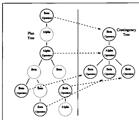
Fig. 3. The plan tree on the left is reduced to the contingency tree on the right by dropping the abstract reasoning nodes.
