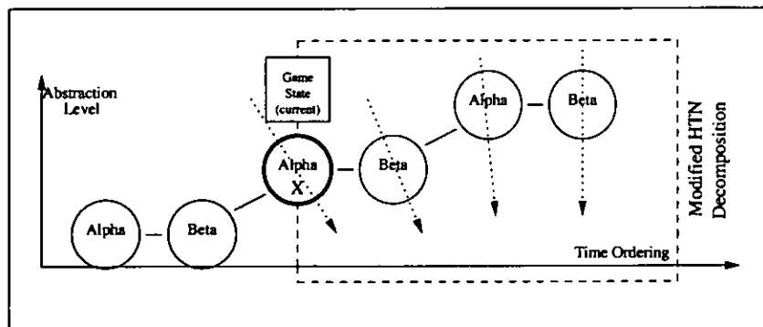
Fig. 5. Goal decomposition in modified HTN planning. The dashed arrows represent the decomposition of goals (eventually) into concrete actions.
