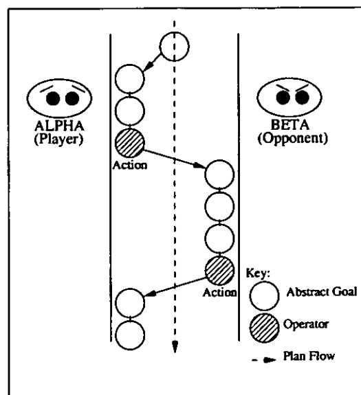
Fig. 1. Planning steps alternating between two agents.
