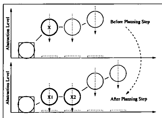
Fig. 2. Plan refinement: abstract goals are expanded to and replaced by sets of subgoals at lower levels of abstraction.
