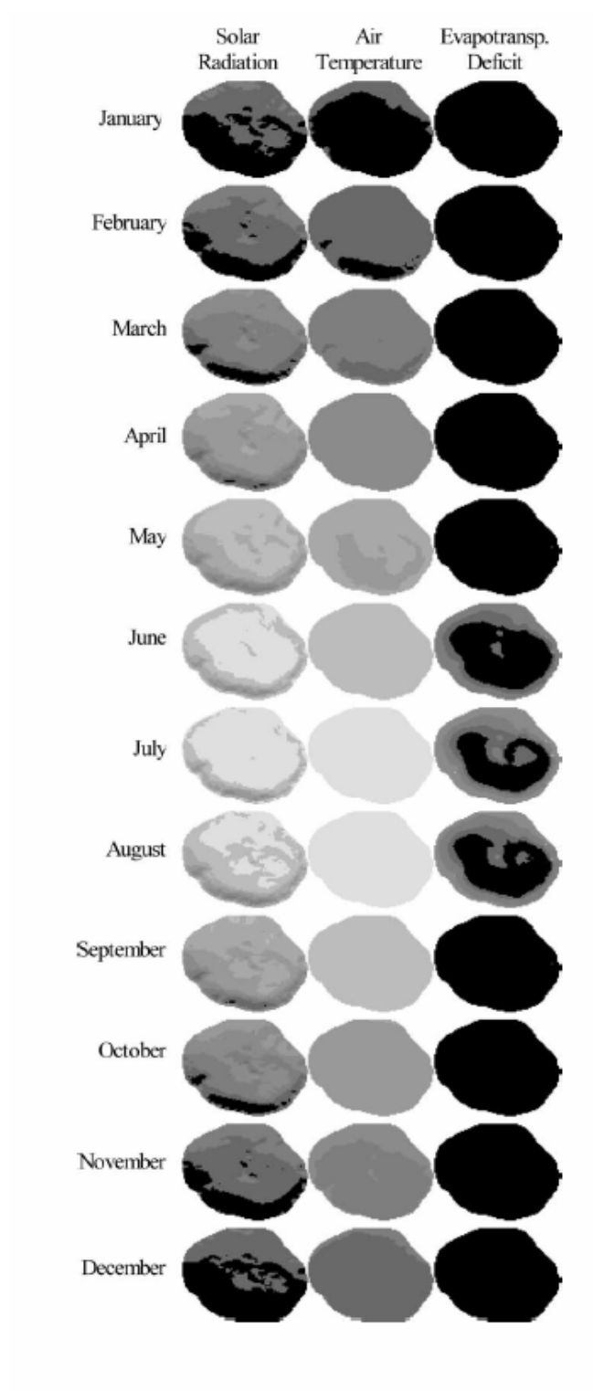
Fig. 2. Modelled environmental characteristics within the Astroni crater from January to December. The maps show tone variations with respect to yearly maxima and minima. For solar radiation, light tones signify high radiation intensities and dark tones signify low radiation intensities. For temperature, light tones signify high temperatures and dark tones signify low temperatures. For evapotranspiration deficit, light tones signify high evapotranspiration deficit and dark tones signify low deficit.
