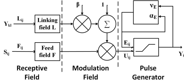
Figure 3: A PCNN neuron model
