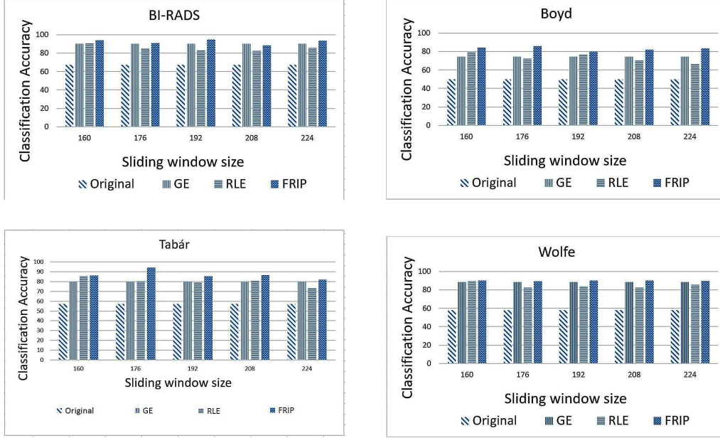
Figure 10: Classification accuracy using different sliding window sizes for all assessment criteria
