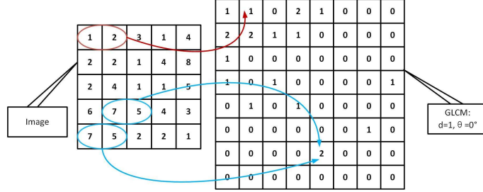
Figure 1: Example of GLCM computation with distance d = 1 and angle \theta = 0^\circ , of an 8 grey level image.
