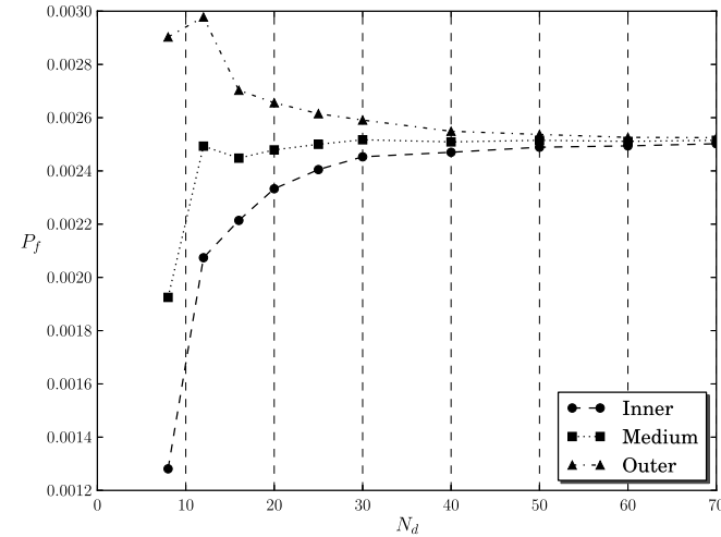
Fig. C.15. Convergence of the probability of failure of the functional requirement for the second set of values.
