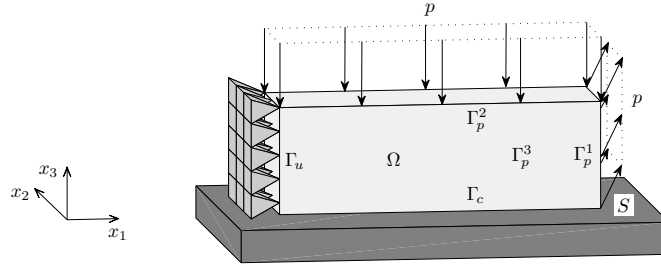
Figure 2: Geometry.
