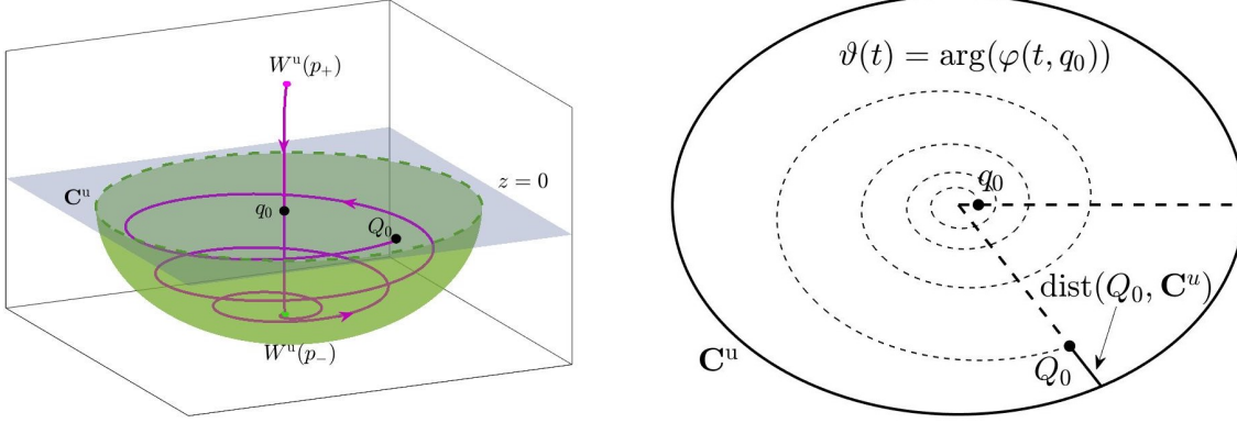
Figure 5: The points q_0 and Q_0 correspond to the first and second intersections of W^u(p_+) with z = 0 . The curve \mathbf{C}^u is given by the first intersection of W^u(p_-) with z = 0 . We need to get appropriate bounds for the angle \theta_0 = \vartheta(t) and for the distance between Q_0 and \mathbf{C}^u . On the left the three dimensional figure, on the right the plane \{z = 0\} .
