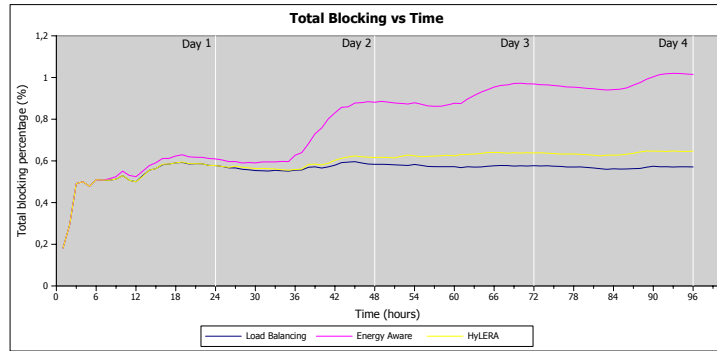
(b) Total blocking vs Time
