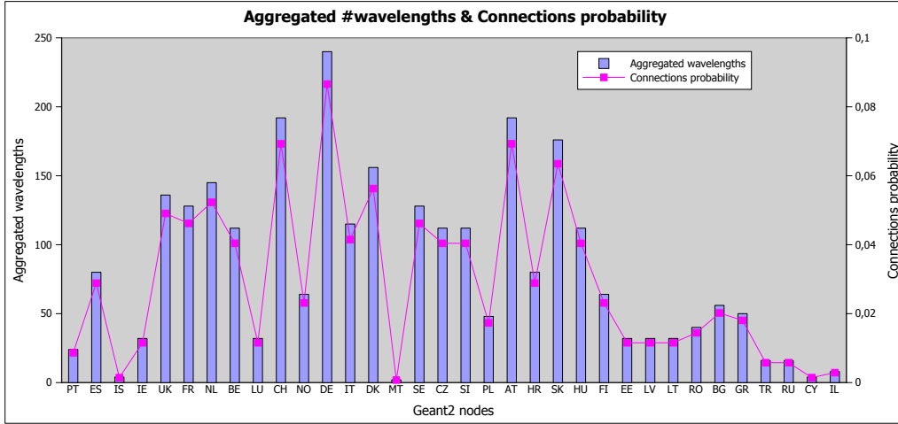
Figure 6: The number of wavelengths of each network node is reported (columns) together with its probability to appear as either source or destination in connection request (dots).
