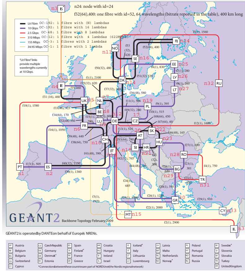
Figure 4: The Geant2 network used in simulations.
