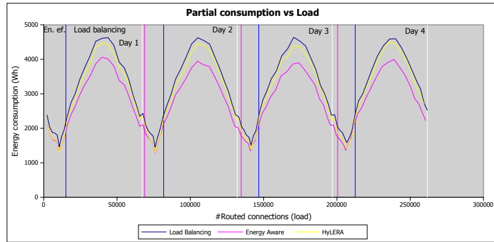
(c) Partial energy consumption vs Load
