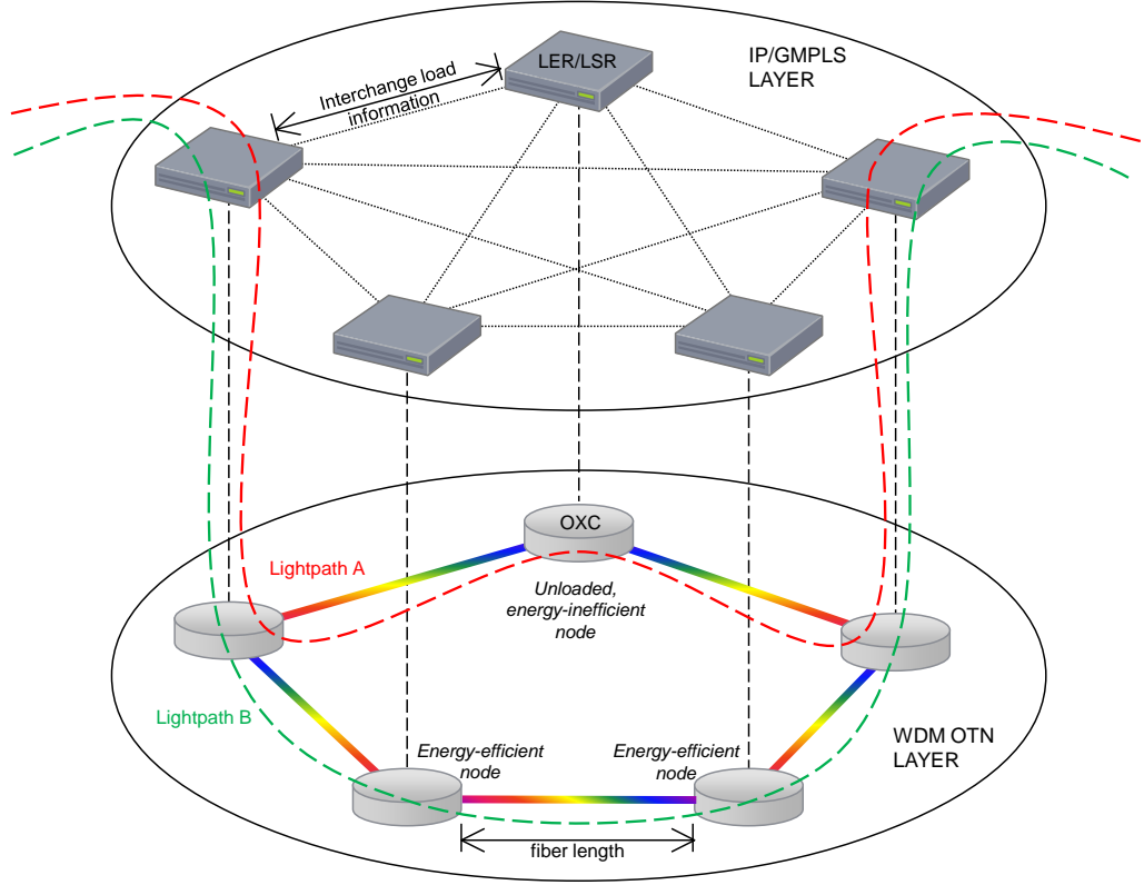
Figure 1: Path selection in a multilayer GMPLS/WDM network according to a pure load-balancing (red line) or a pure energy-efficient (green line) criteria; the optimal selection depends on the current network traffic state.
