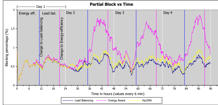
(a) Partial block vs Time
