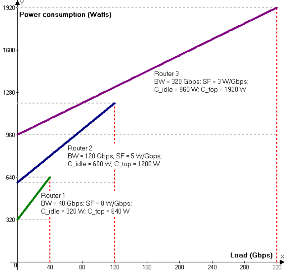
Figure 2: The energy consumption of three routers with different aggregated bandwidth (BW) and scaling factors (SF) are represented.
