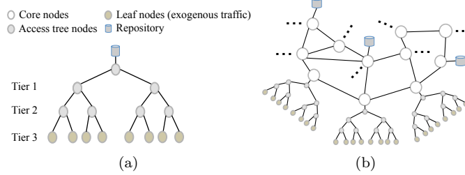
Figure 4: Network Topologies: (a) 4-level binary tree, (b) CDN-like.
