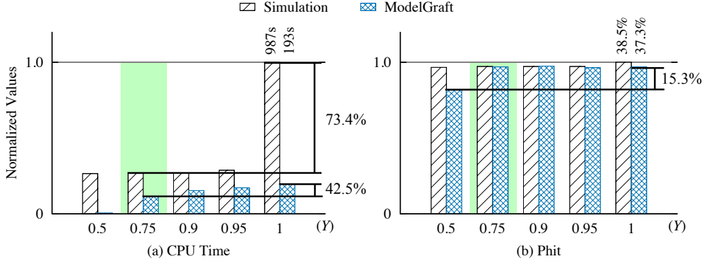
Figure 7: Consistency parameter Y sensitivity: very large-scale scenario for NDN Testbed topology with, M = R = 10^9, C = 10^6, \Delta = 10^5 , LCE. Normalized (a) CPU time and (b) p_{hit} when the system converges to steady-state. Default value highlighted in green.
