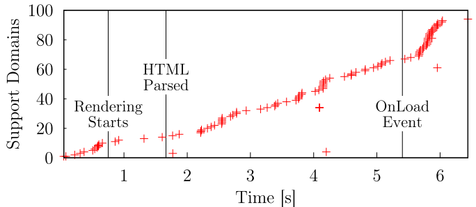
Fig. 2. Support domain flows for a visit to www.bbc.co.uk . The browser contacted 94 support domains (y-axis) during 6 seconds (x-axis). Notable browser events are reported as vertical lines.
