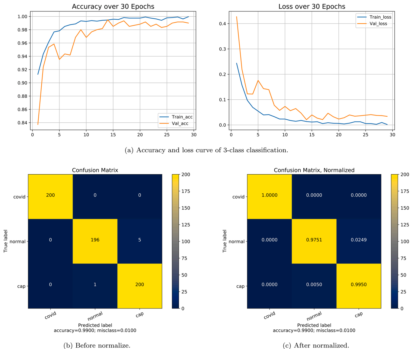
Fig. 17. Classification performance results on 3-class using fold-1 chest ct-scan dataset.
