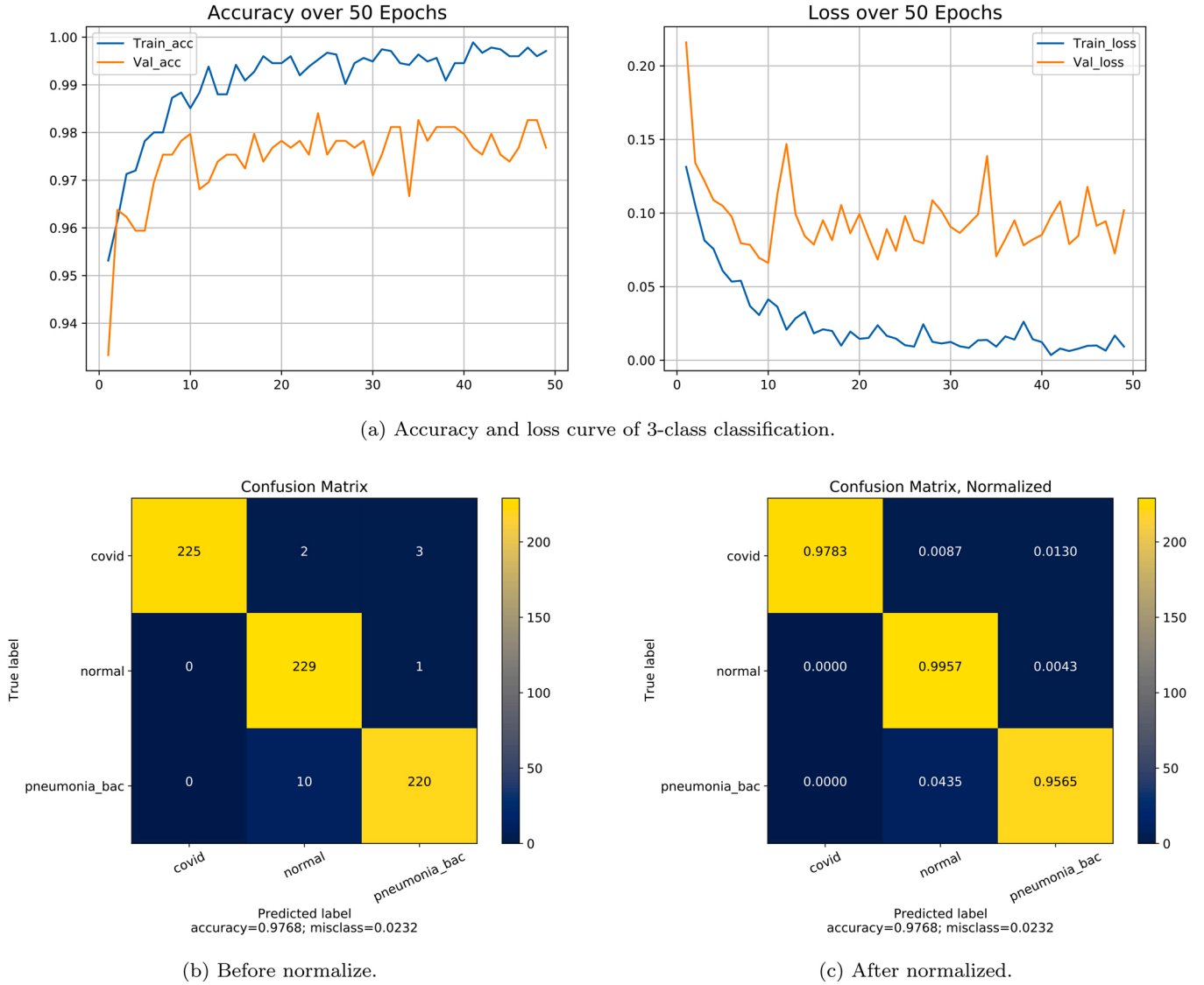
Fig. 13. Classification performance results on 3-class using fold-3 chest x-ray datasets.
