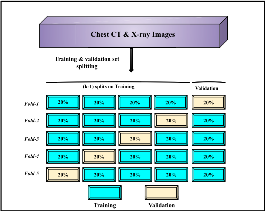
Fig. 11. Schematic illustration of five -fold cross validation approach.
