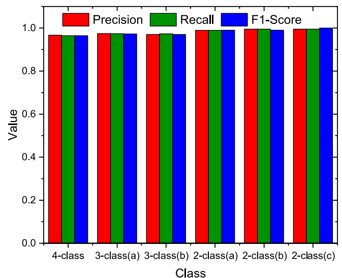
Fig. 15. Average precision, recall &amp; f1-score of 4-class, 3-class (a. covid vs pneu_bac vs normal, b. covid vs pneu_vir vs normal), 2-class (a. covid vs pneu_vir, b. covid vs normal, c. covid vs pneu_bac).
