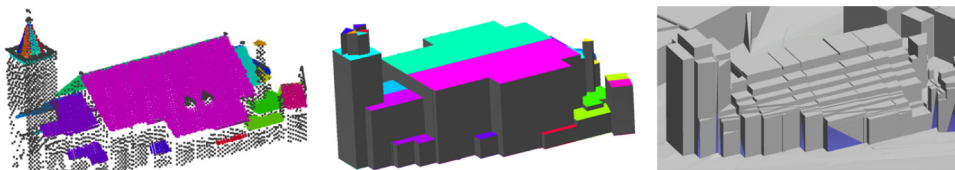
Fig. 10. Point cloud with plane segmentation (left), LoD1.3 model with our 3D approach (middle) and LoD1.3 model with our 2D approach (right).
