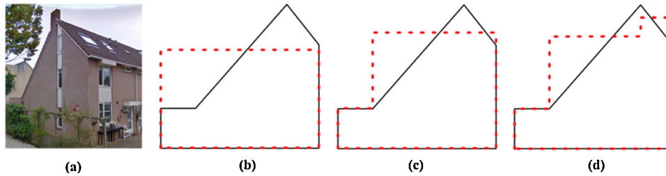
Fig. 11. Three different LoD1.3 modelling possibilities (b,c,d) for a building with an asymmetric gabled roof (a).
