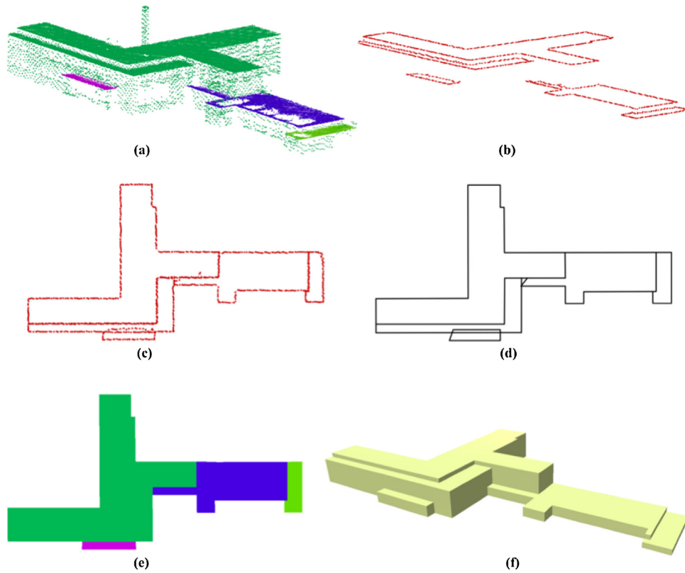
Fig. 9. The steps in our improved method to reconstruct LoD1.3 buildings.
