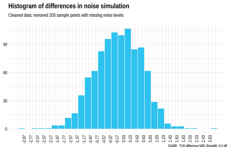
Fig. 17. Histogram of differences in results of noise simulation between the simulation based on the original input data and based on our generated input data.
