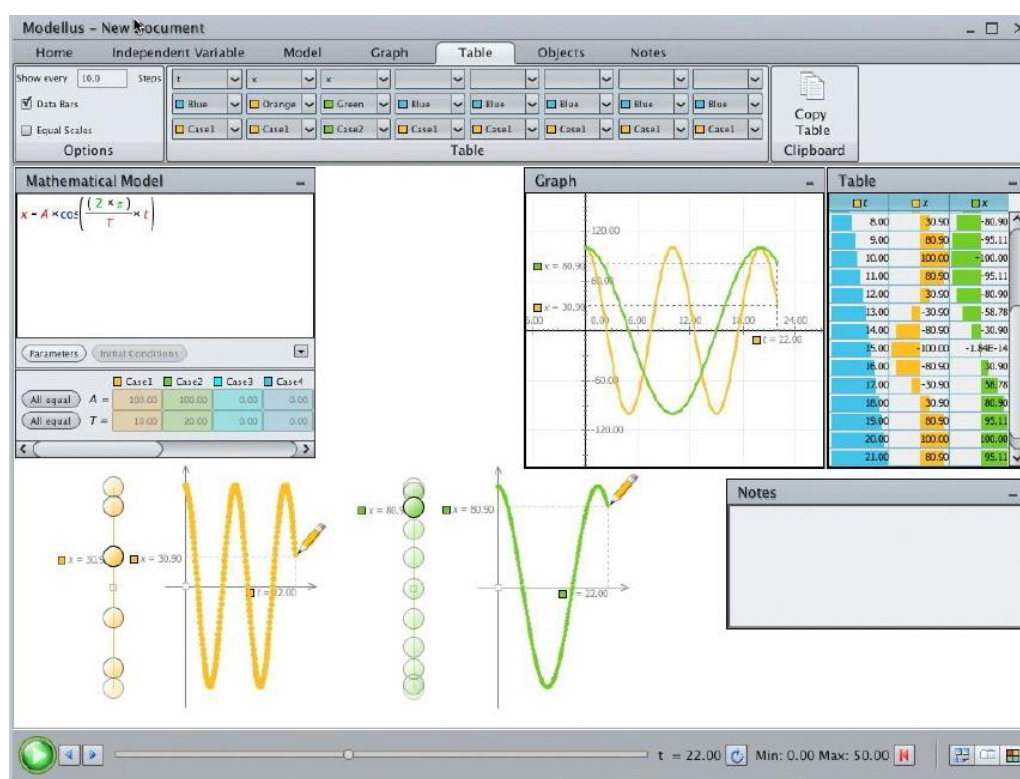
Fig. 1 A Modellus file illustrating simple harmonic motion, using functions and two sets of different parameters. This model can also be made using differential equations or iterative equations.
