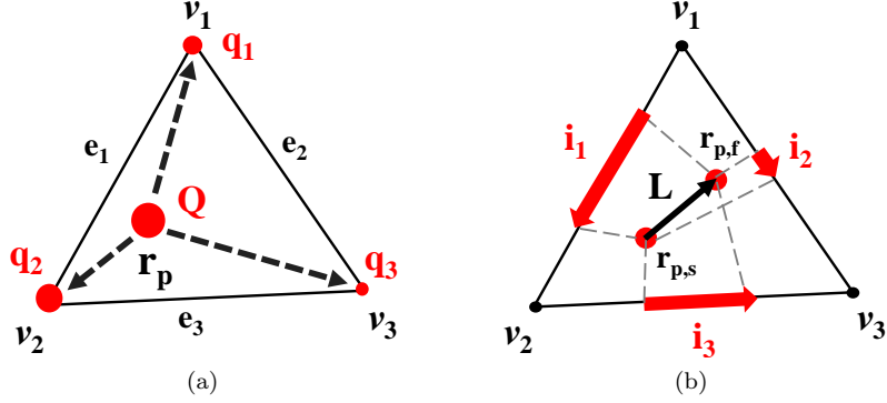
Figure 2: Scatter step: (a) Nodal charge assignment from a charged particle placed at \mathbf{r}_p with local numbering of vertices and edges and (b) Current assignment due to charge movement from \mathbf{r}_{p,s} to \mathbf{r}_{p,f} during \Delta t with default directions for currents.
