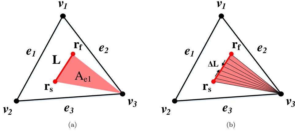
Figure A.12: Geometric illustration of the weight assigned to Whitney 1-forms representing a segment \mathbf{L} in a 2-D simplex: (a) In red color is the area A_{e1} associated with the Whitney 1-form on e_1 (edge 1) that represents \mathbf{L} . The associated weight is given by A_{e1}/A , where A is the total area of the triangle composed of \nu_1, \nu_2 , and \nu_3 . A similar construction can be made for the other two edges e_2 and e_3 . (b) Area represented by a sum of small triangles. See the main text for more details.
