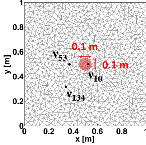
Figure 8: Mesh with 2539 edges and three selected nodes \nu_{10} , \nu_{53} , and \nu_{134} . A total of 4 \times 10^3 negatively charged particles are initially placed in the red circle, uniformly distributed.
