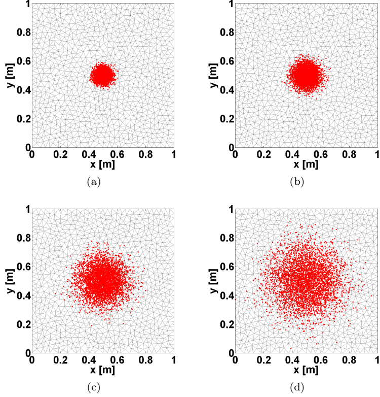
Figure 9: Distribution of 4 \times 10^3 particles with initial Maxwellian distribution, and zero initial fields. The particle distribution is shown at different time instants ( \Delta t = 0.01 ns): (a) t = 10^4 \Delta t , (b) t = 2 \times 10^4 \Delta t , (c) t = 4 \times 10^4 \Delta t , and (d) t = 6 \times 10^4 \Delta t .
