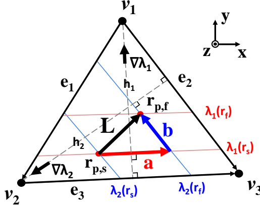
Figure B.13: An arbitrary particle path \mathbf{L} during \Delta t and associated parameters in the xy -plane.
