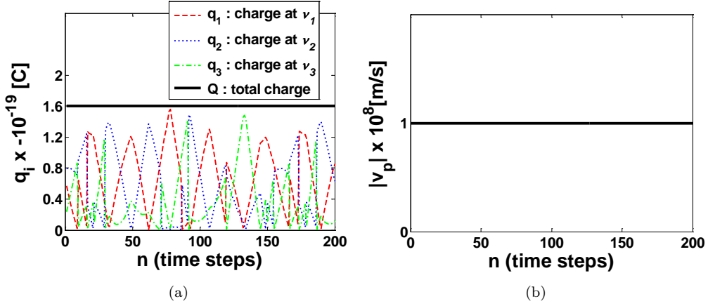
Figure 6: Charge and energy conservation: (a) Distributed amounts of charge to local vertices and their sum at all time steps and (b) Absolute value of the particle velocity at all time steps.
