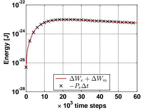
Figure 10: Numerical verification of energy conservation with a plot of the left hand side and the right hand side of (48) for all time steps.
