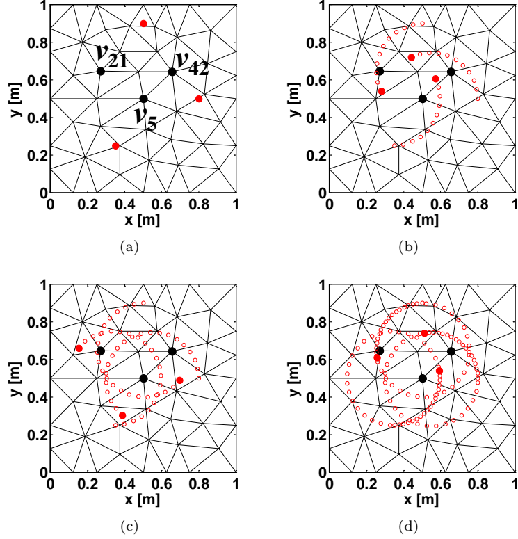
Figure 7: Movement of three particles in the uniform static magnetic field at different time instants ( \Delta t = 0.1 ns): (a) t = 0 , (b) t = 50\Delta t , (c) t = 100\Delta t , and (d) t = 200\Delta t .
