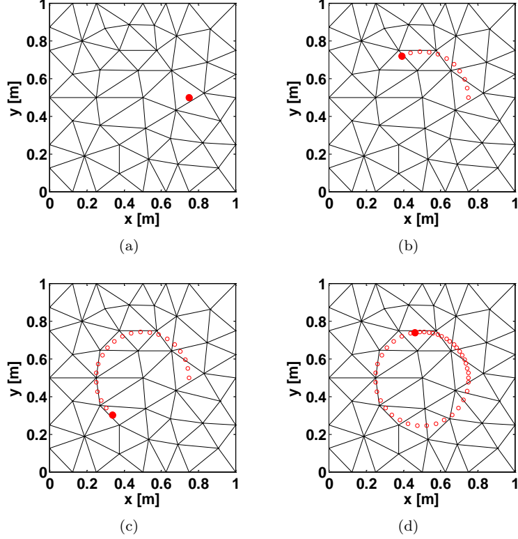
Figure 5: Movement of a single particle in the uniform static magnetic field at different time instants ( \Delta t = 0.1 ns): (a) t = 0 , (b) t = 50\Delta t , (c) t = 100\Delta t , and (d) t = 200\Delta t .
