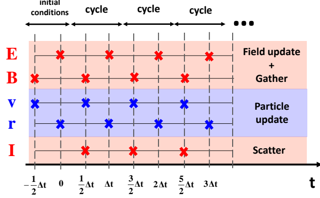
Figure 4: Full time-update procedure for the charge-conserving PIC algorithm.
