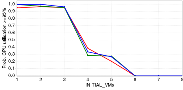
Fig. 2. PRISM results for P=? [F_{util} \geq 95] ("periodic" load)
