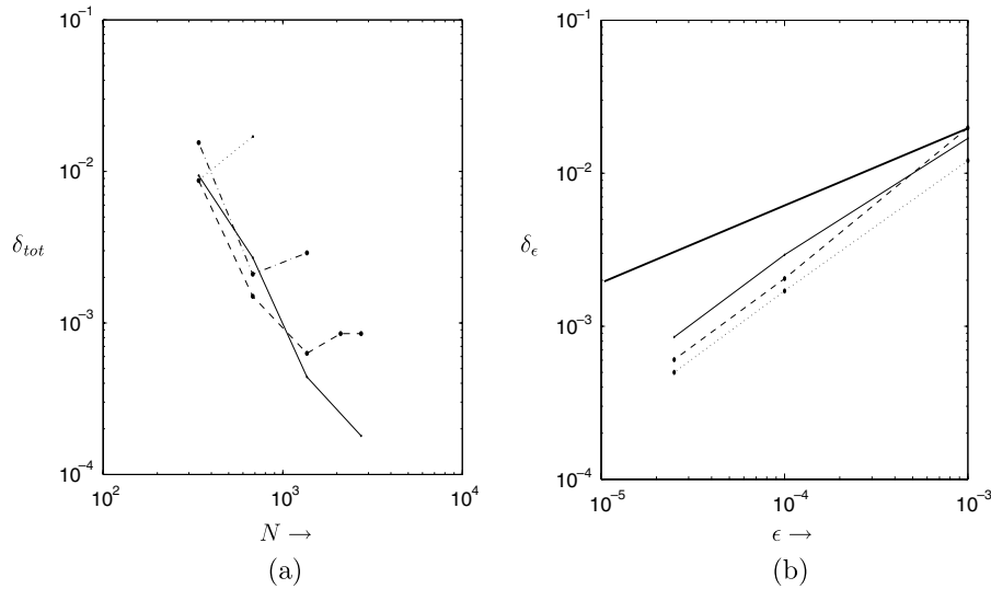
Fig. 18. Total error \delta_{tot} versus number of Fourier modes N at t = 0.8 , \epsilon = 10^{-3} (dots), \epsilon = 10^{-4} (dashed-dot), \epsilon = 2.5 \times 10^{-5} (dashed) and \epsilon = 10^{-8} (solid) (a). Modelling error versus \epsilon computed at t = 0.4 (dots), t = 0.5 (dashed) and t = 0.8 (solid) and theoretical upper bound (b).
