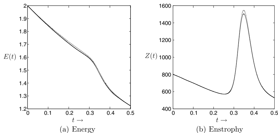
Fig. 13. Comparison of E(t) (a) and Z(t) (b) between the CVS run on 1024^2 -grid, \delta t = 5 \times 10^{-5} , and penalization parameter \epsilon = 10^{-4} (solid) and the Chebyshev run with 640^2 modes (dots) and \delta t = 1.25 \times 10^{-5} .
