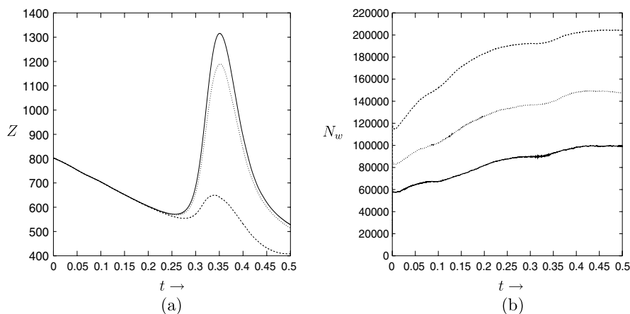
Fig. 16. Enstrophy versus time for three different values of the penalization parameter \epsilon = 10^{-2} (dashed), \epsilon = 10^{-3} (dots) and \epsilon = 10^{-4} (solid), threshold \tilde{\epsilon}_0 = 10^{-5} is fixed (a). Number of wavelet coefficients N_w with security zone for three different values of the threshold \tilde{\epsilon}_0 = 10^{-4} , \tilde{\epsilon}_0 = 10^{-5} and \tilde{\epsilon}_0 = 10^{-6} with penalization parameter \epsilon = 10^{-4} fixed (b).
