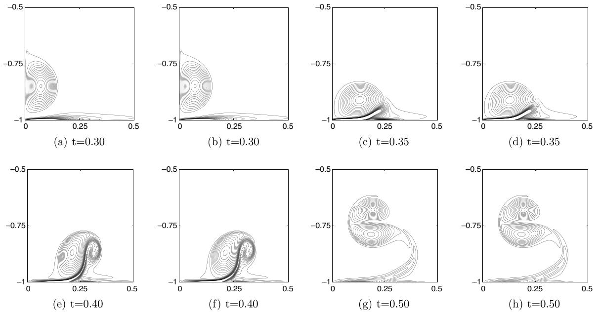
Fig. 5. Contour plots of the vorticity of a normal dipole–wall collision with Re = 1000 . Panels (a, c, e, g) show mollified Fourier projection using 1364 \times 1364 active Fourier modes, \delta t = 10^{-5} and \epsilon = 2.5 \times 10^{-5} with an implicit treatment of Darcy drag. Panels (b, d, f, h) show the Chebyshev–Fourier benchmark computation with 1024 Chebyshev modes and 2048 Fourier modes. Contour levels are drawn for -270, \dots, -50, -30, -10, 10, 30, 50, \dots, 270 .
