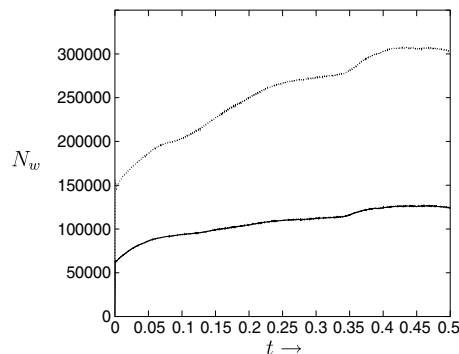
Fig. 12. Time evolution of the number of wavelet coefficients N_w with (dots) and without (solid) security zone for CVS computation on 1024^2 grid with \delta t = 5 \times 10^{-5} .
