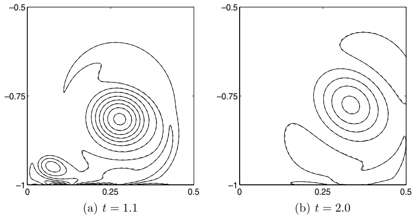
Fig. 9. Contour plots (dashed) of the vorticity for \epsilon = 10^{-8} with 1364 \times 1364 active Fourier modes and Chebyshev–Fourier benchmark computation (solid). Contour levels are drawn for, ..., -50, -30, -10, 10, 30, 50, ...
