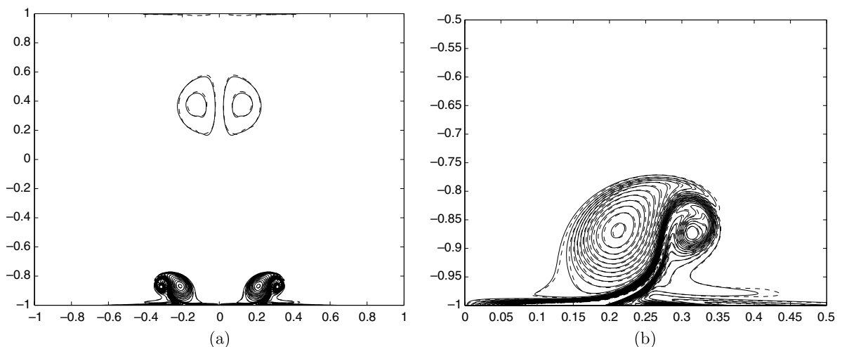
Fig. 10. Isolines (dashed) of \omega drawn for -270, ..., -50, -30, -10, 10, 30, 50, ..., 270, comparison of CVS simulation on 1024^2 grid and \delta t = 5 \times 10^{-5} , with the Chebyshev run with 640^2 modes and \delta t = 1.25 \times 10^{-5} (solid) at t = 0.4 . Left: total domain. Right: zoom in.
