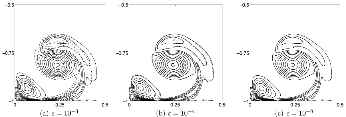
Fig. 17. Contour plots (dashed) of the vorticity after the second collision at t = 0.8 for different values of the penalization parameter \epsilon with respect to the benchmark simulation (solid). Contour levels are drawn for -270, -250, \dots, -30, -10, 10, 30, 50, \dots, 250, 270 . Number of active Fourier modes 682^2 (a), 1364^2 (b) and 2730^2 (c), time-step is fixed to \delta t = 10^{-5} .
