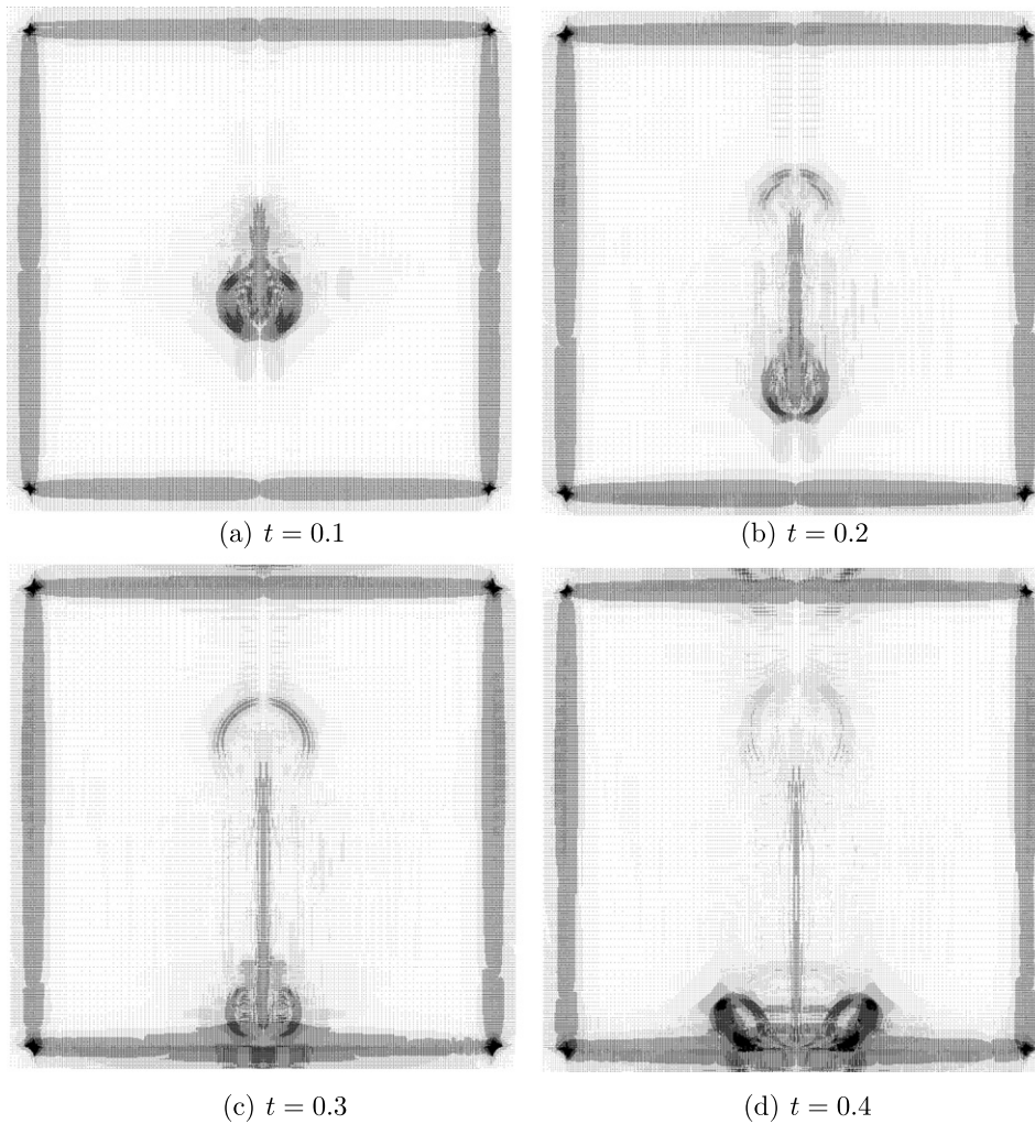
Fig. 11. Adaptive grid at t = 0.1, 0.2, 0.3 and 0.4 for CVS computation with 1024 grid points in both directions. The number of wavelets are 93,674, 104,711, 112,065 and 124,364 for t = 0.1, 0.2, 0.3 and 0.4 , respectively.
