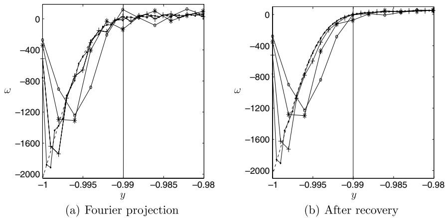
Fig. 6. Cross-section of the vorticity along the line x = 0.083 at t = 0.35 , Chebyshev–Fourier benchmark result (dashed) and implicit scheme (solid). \delta t = 10^{-5} , \epsilon = 2.5 \times 10^{-5} , with different number of active Fourier modes: 512^2 (open circles), 682^2 (stars), 1364^2 (plus signs) and 2730^2 (closed circles).
