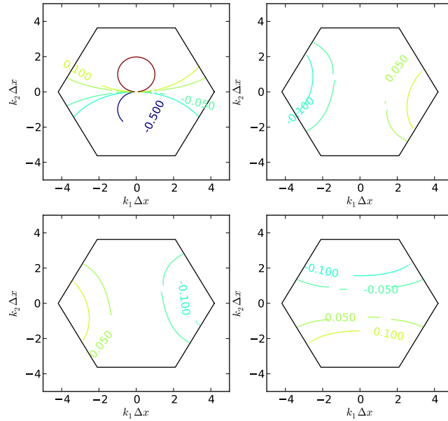
Figure 6: Contour plots showing \omega \times 10^6 obtained from the solutions of equation (27), with parameters f_0 = 1.0 \times 10^{-4} , \beta = 1.0 \times 10^{-12} , \Delta x = 1.0 \times 10^5 and c^2 = 1.0 \times 10^5 (these parameters are the same as those used in Thuburn (2008)). f increases in the x -direction relative to the mesh. The lowest branch of the dispersion relation is shown top-left. The other branches are aliased higher values of \mathbf{k}\Delta x .
