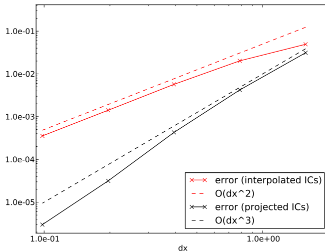
Figure 1: Plot showing convergence rates for the P1_{DG} - P2 discretisation applied to the linear rotating shallow-water equations on an f -plane. The test problem is a single propagating sinusoidal wave in periodic boundary conditions, with the L_2 error in the free surface elevation computed after the wave has propagated all the way around the periodic domain. Second-order convergence for the free surface elevation is obtained when the initial conditions for velocity are obtained by collocation at node points; third-order convergence for the free surface elevation is obtained when the initial conditions are obtained by collocation with a quadratic P2 basis for velocity and reduced to the P1_{DG} space by L_2 projection.
