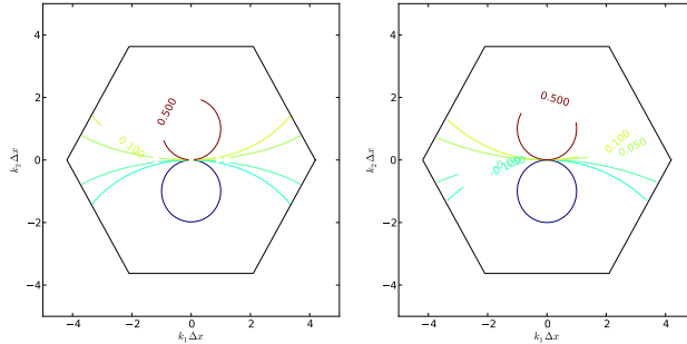
Figure 7: Comparison between the lowest branch of the discrete dispersion relation (left) and the exact dispersion relation (right). f increases in the y -direction relative to the mesh.
