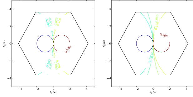
Figure 5: Comparison between the lowest branch of the discrete dispersion relation (left) and the exact dispersion relation (right). f increases in the y -direction relative to the mesh.
