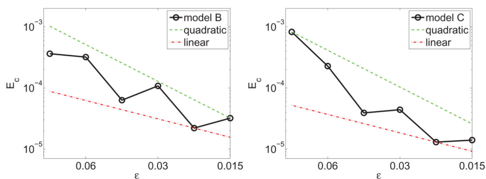
Figure 2. Convergence study showing a super-linear decrease of the accumulated stretching E_c in Eq. (55), as a function of the interface thickness \epsilon , for models B (left) and C (right).
