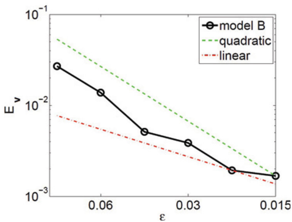
Figure 1. Convergence study showing a super-linear decrease of the instantaneous stretching E_v in Eq. (54) as a function of the interface thickness \epsilon for model B.
