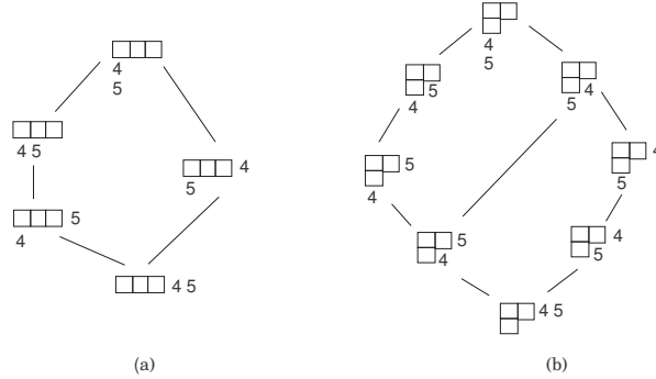
FIGURE 3. An illustration of the skew orders on SYT_n^\mu for n = 2 . When \mu is (a) rectangular and (b) nonrectangular, SYT_2^\mu has its proper part homotopy equivalent to a 0-dimensional sphere and a point respectively.
