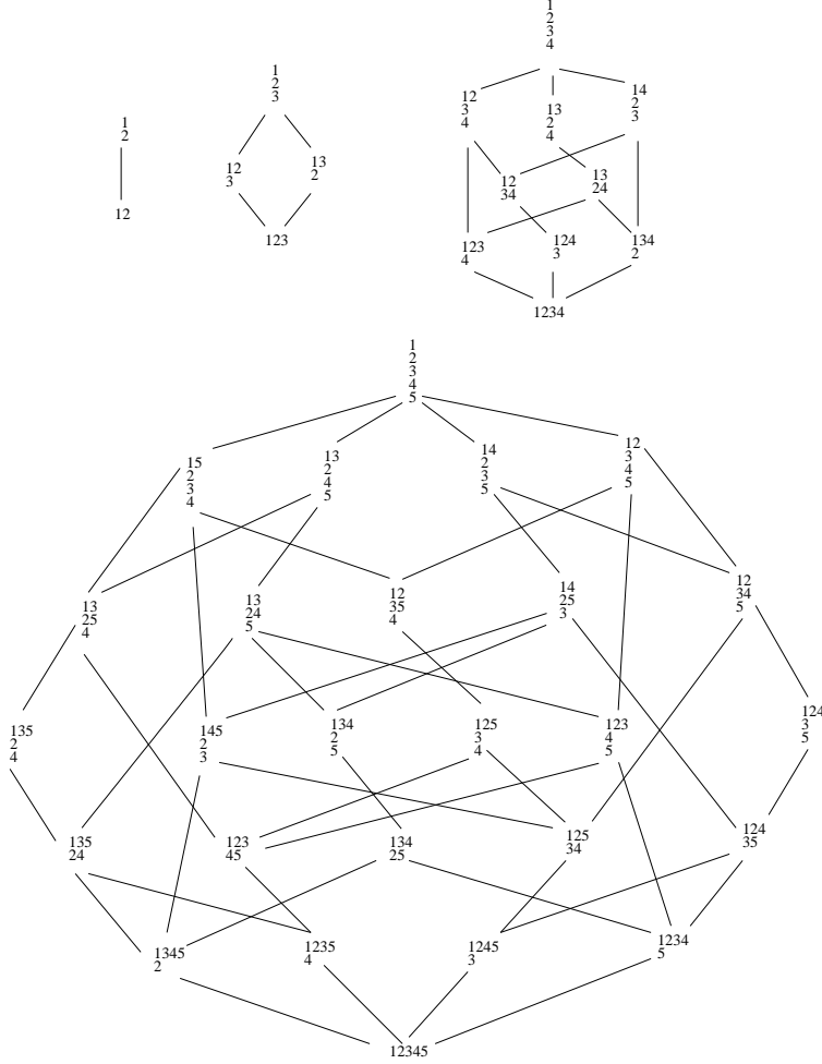
FIGURE 1. Chain, the weak, KL and geometric order on SYT_n , which coincide for n = 2, 3, 4, 5 (but not in general).
