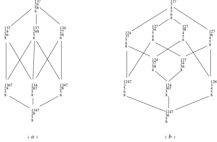
FIGURE 2. (a) An interval in (SYT_8, \leq_{chain}) and (b) an interval in SYT_8 ordered with \leq_{weak} , \leq_{KL}^{op} and \leq_{geom} having Möbius function 2 and -2 respectively.
