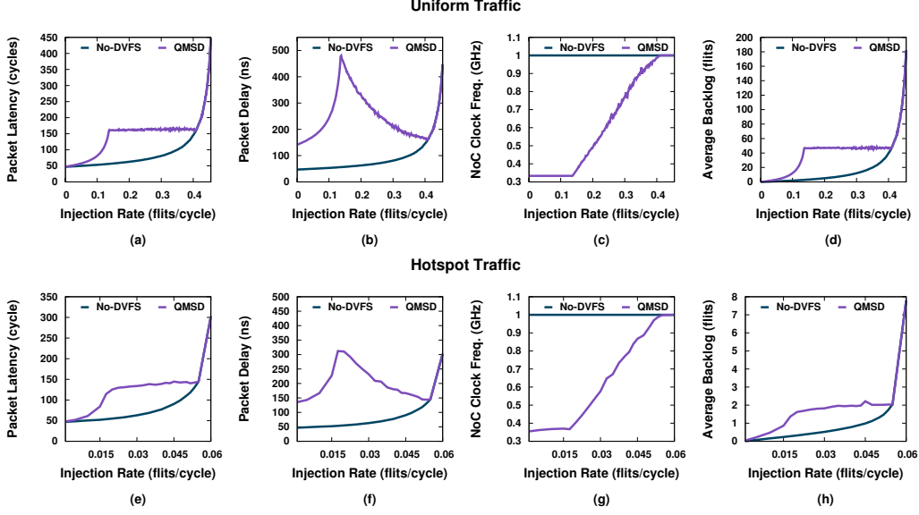
Figure 7: Performance figures without DVFS and with a QMSD policy in a 4×4 NoC.
