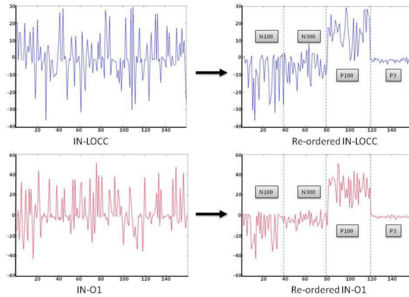
Figure 6. (Left) IN-LOCC and IN-O1 point-sequence curves prior to grouping and reordering. (Right) Labeled curves for metrics IN-O1 and IN-LOCC after grouping/reordering.
