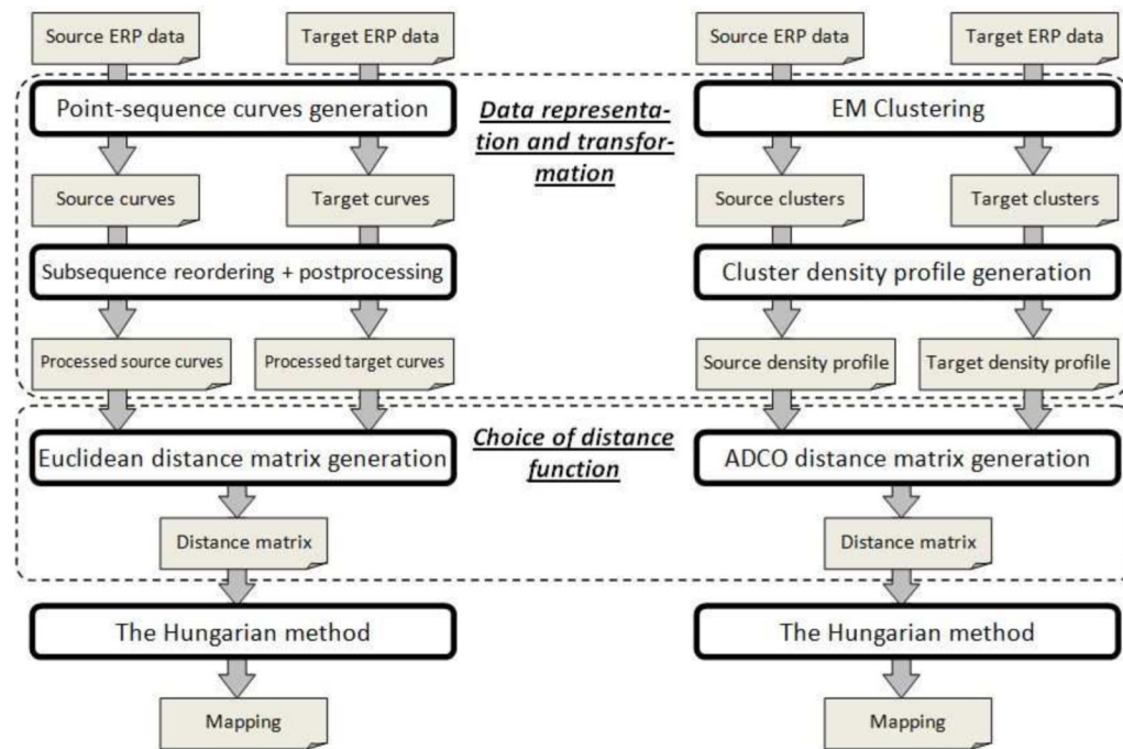
Figure 3. Flowchart of the proposed approach. (left—metric matching, right—pattern matching.)
