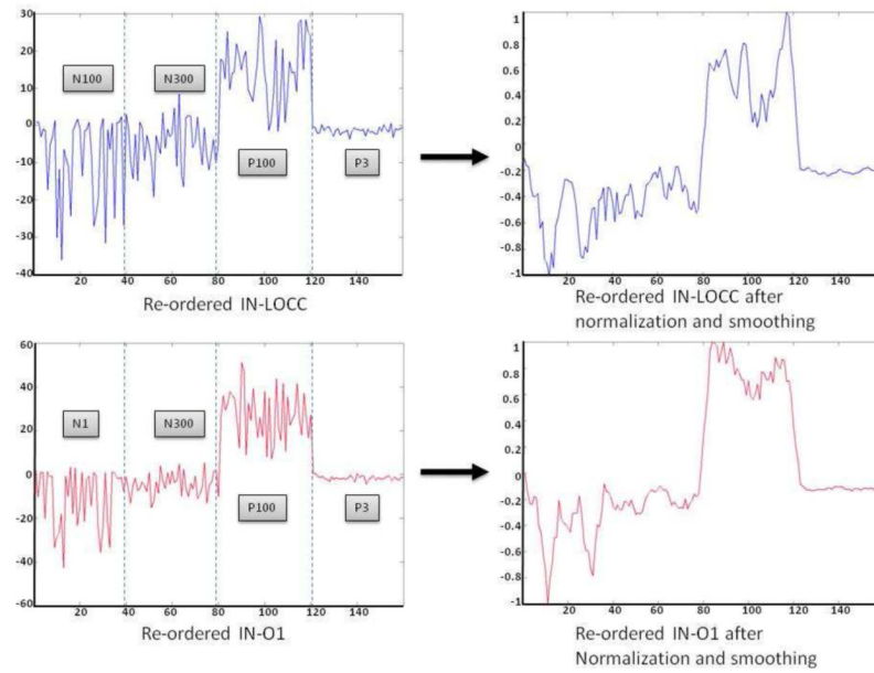
Figure 7. After normalization, smoothing, and interpolation of point-sequence curves in Fig. 6
