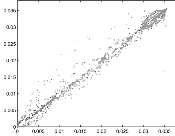
Fig. 4. Scatter plot of the Stand Pipe Pressure ( x -axis is value of Stand Pipe Pressure at time t and y -axis is value of Stand Pipe Pressure at time t + 1 ) for the two classes in the oil production data (black “+” is tripping in class and gray “o” is tripping out class). The conditional correlation of this attribute over time is evident.
