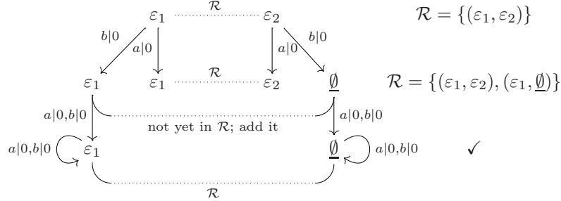
Figure 5: Bisimulation construction
