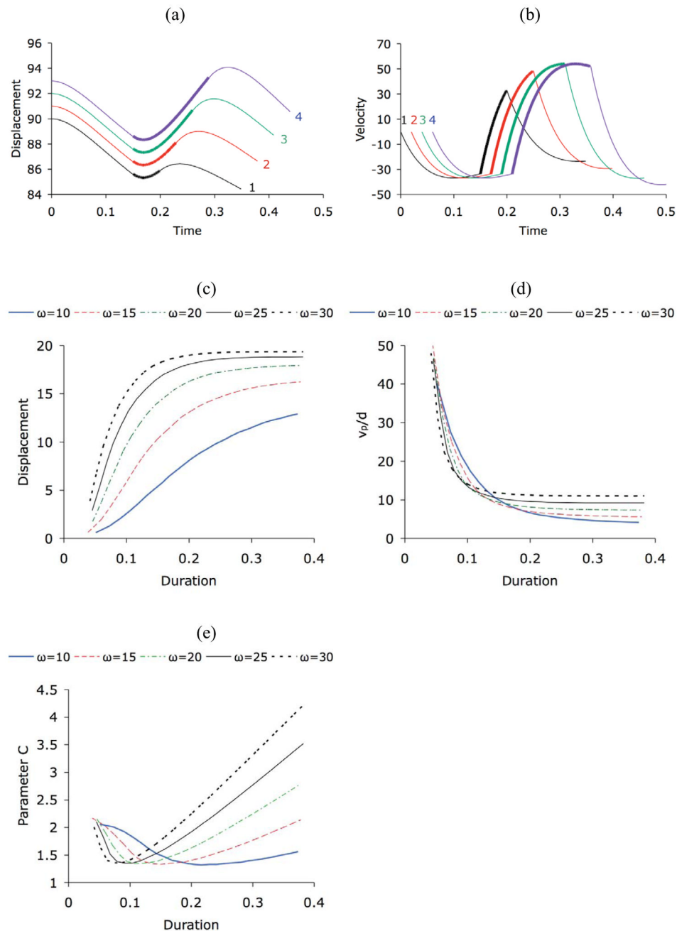
Fig. 9. (a) Simulated movement trajectories based on a critically damped second-order linear system defined by equation [5]. See text for details about the parameters used. (b) Velocity profiles of the trajectories in (a). (c) Simulated displacements as a function of duration at different stiffness levels indicated by \omega_n . (d) Simulated v_p/d ratios as a function of duration at different stiffness levels. (e) Simulated parameter C (peak-velocity/average-velocity) as a function of duration at different stiffness levels.
