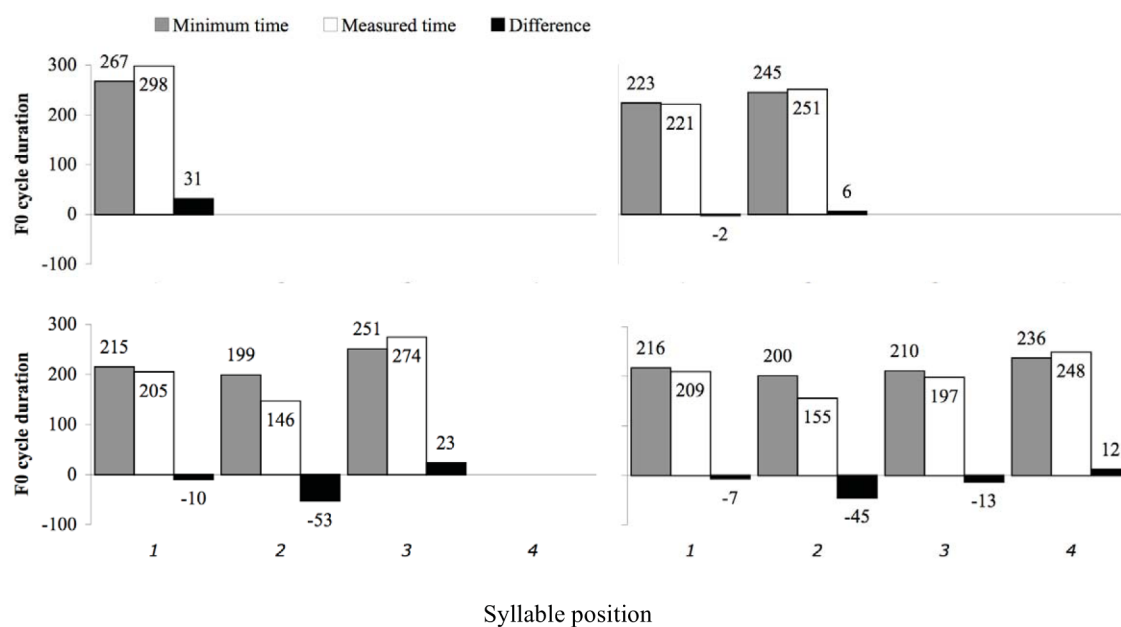
Fig. 8. Up-down cycle duration shown in Figure 4a (white bars), minimum time needed for making the amount of F_0 displacement at each syllable position shown in Figure 4b, computed with equations [3] and [4] (grey bars), and the difference between the two (measured – predicted) (dark bars). The separate bar clusters show values for the 1–4 syllable sequences, respectively.
