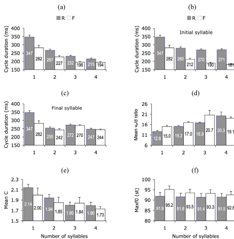
Fig. 3. Various measures of all-R and all-F sequences as a function of phrase length and tone. (a) Mean up-down cycle duration. (b) Mean up-down cycle duration of the initial syllable. (c) Mean up-down cycle duration of the final syllable. (d) Mean v_p/d ratio. (e) Mean C. (f) Mean maxF 0
