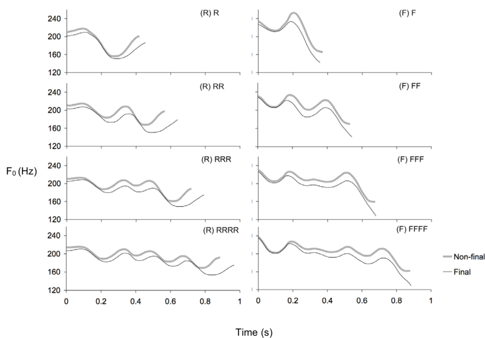
Fig. 2. Effects of location in sentence and phrase length on Mean F_0 curves of all-R and all-F sequences. Thin line — sentence final; thick line — non-final.
