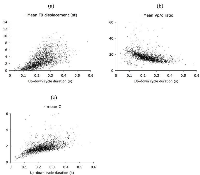
Fig. 6. Scatter plots of F_0 displacement (a), mean v_p/d ratio (b) and mean C (c) as functions of up-down cycle duration.
