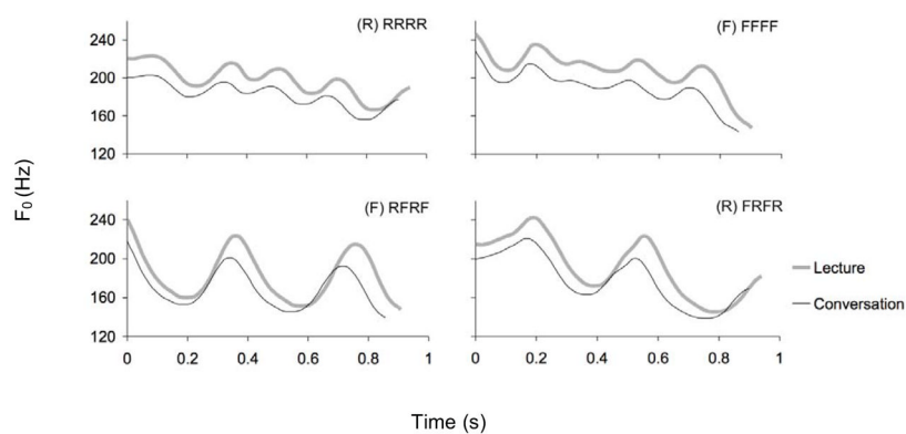
Fig. 1. Mean F_0 curves under the effects of speaking mode and articulatory pressure. Thick line — Mean F_0 curves of all-R, all-F, RF and FR sentences in lecture mode. Thin line — Mean F_0 curves in conversation mode.
