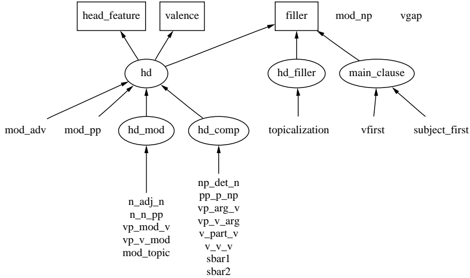
Figure 2: The Rule Hierarchy (with PRINCIPLES shown in boxes, structures in ovals, and rules without frame). Note that the mod_np rule (a unary rule which transforms temporal NPs into verbal modifiers) and the vgap rule (a rule which introduces verbal gaps) are exceptional in that they do not inherit from general principles.
