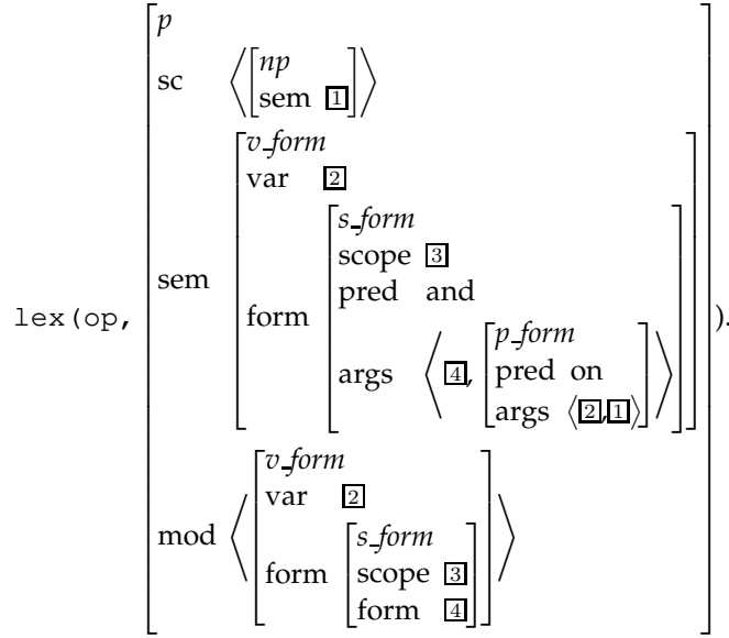
Figure 17: Adverbial semantics for prepositions.
