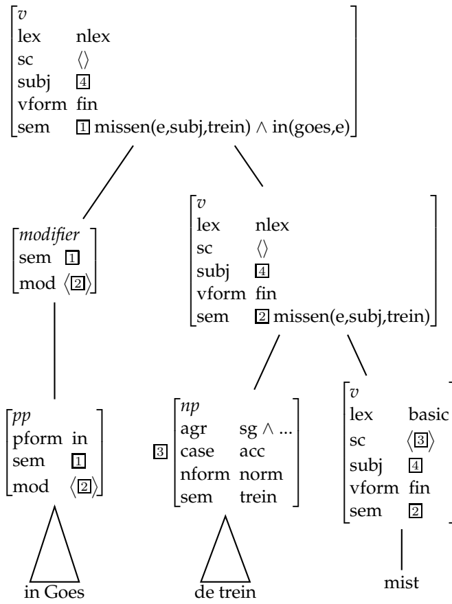
Figure 6: (dat Rob) in Goes de trein mist (that Rob misses the train in Goes)
