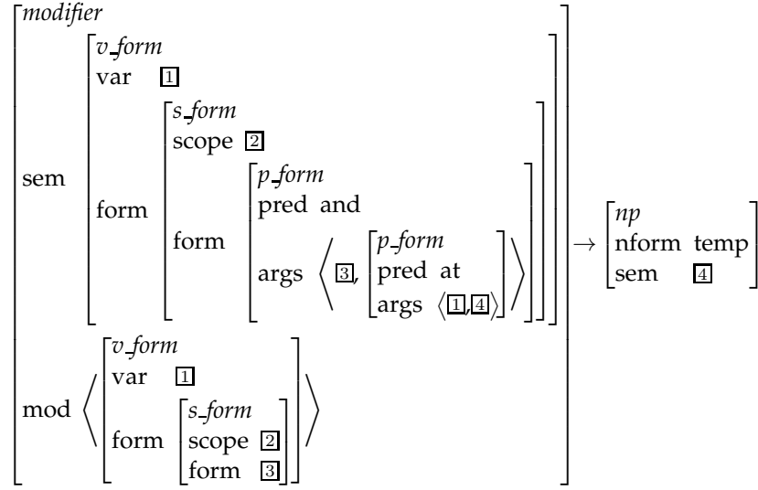
Figure 18: Rule mod_np to treat temporal noun phrases as modifiers.
