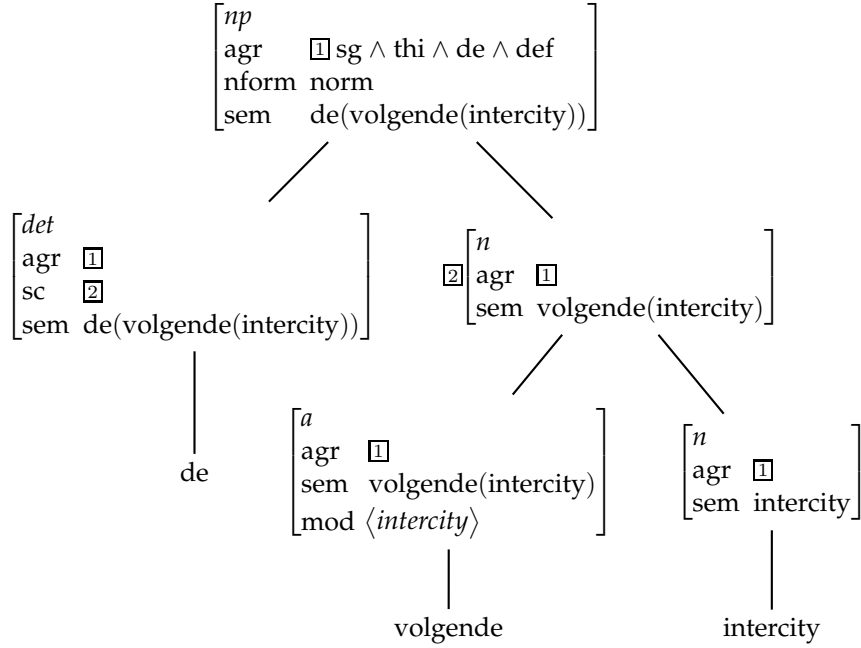
Figure 4: de volgende intercity (the next intercity)
