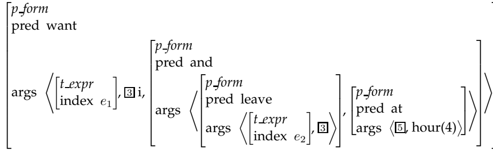
Figure 13: QLF for 'Ik wil om ongeveer vier uur vertrekken' (I want to leave at about four o'clock)
