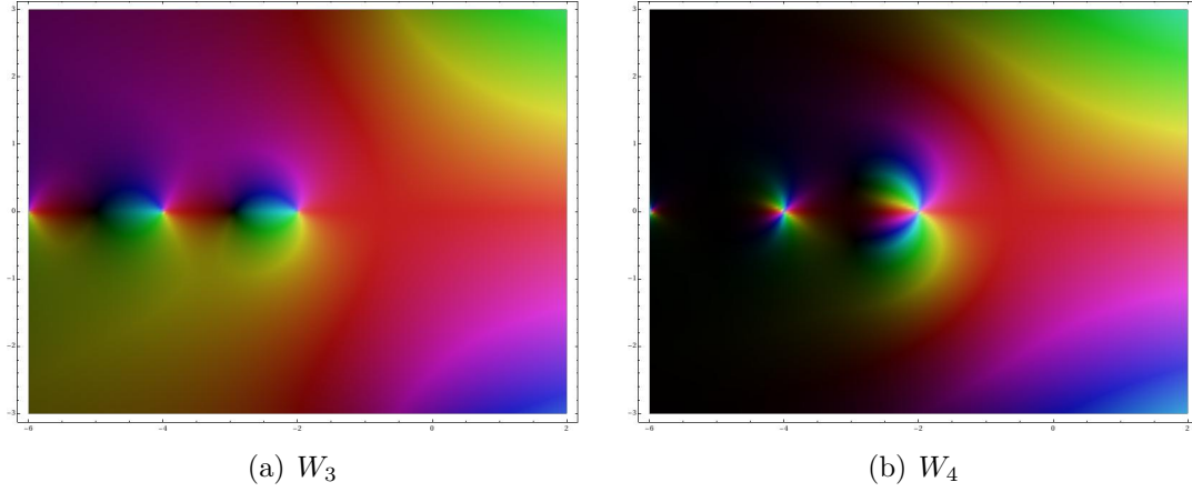
Figure 2: W_3 via (24) and W_4 via (25) in the complex plane.
