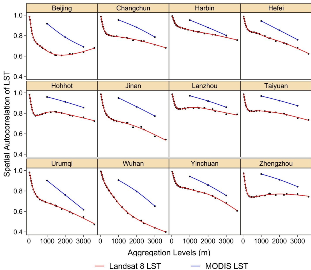
Figure S3. Effects of data aggregation levels on SA of Landsat 8 LST and MODIS LST.
