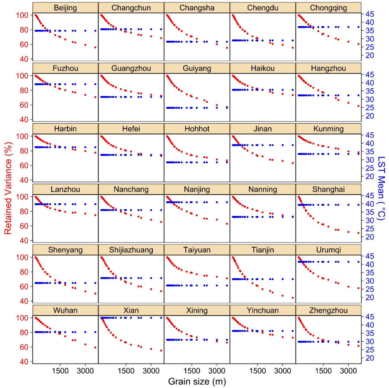
Figure S1. The mean and variance of LST of 30 sample cities for different aggregation levels.
