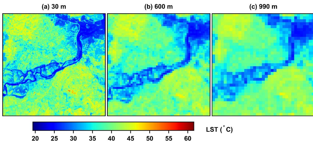
Figure S2. The LST in Harbin for different aggregation levels: 30 m (a), 600 m (b), 990 m (c).
