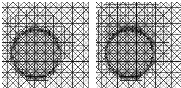
FIGURE 7.3. Effect of coarsening for Approach I and \varepsilon = 10 , \gamma_h/\Gamma_h = \sqrt{0.2}(\sqrt{0.1}) .
