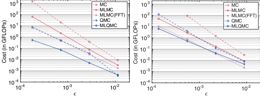
FIGURE 3. Cost to obtain a relative standard error less than \varepsilon in the 1D example. The covariance parameters are \nu = 1 and \sigma^2 = 1 , as well as \lambda_C = 1.0 (left) and \lambda_C = 0.1 (right), respectively. The estimates for C_{\text{bal}} are 0.38 (left) and 1.78 (right), respectively.
