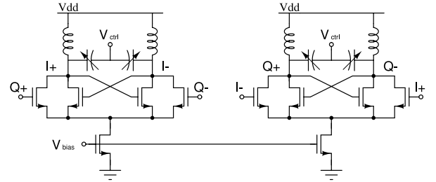
Fig. 7 Quadrature-coupled LC-VCO.
