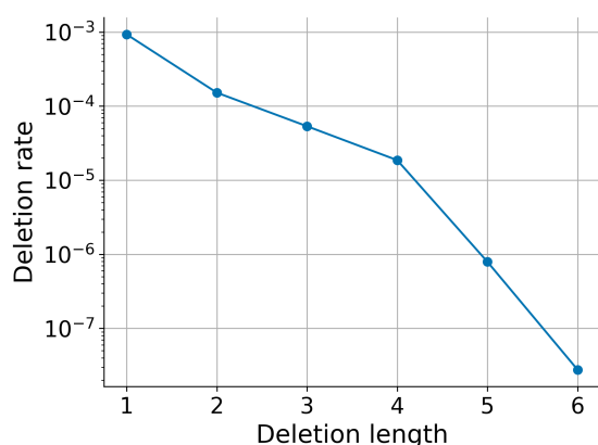
Figure 12: Deletion length distribution (see 2.2.2.4).
