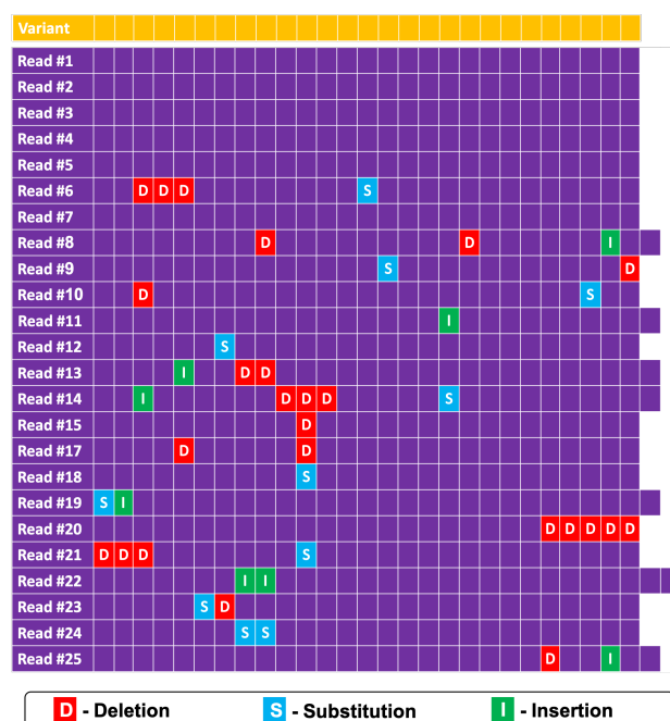
Figure 1: An example of 25 reads (in purple) aligned to a variant of length 27 (in yellow). For each read, the locations of the deletions, substitutions, insertions are marked in red, blue, green, respectively. This alignment output forms the basis of the analysis performed by SOLQC.
