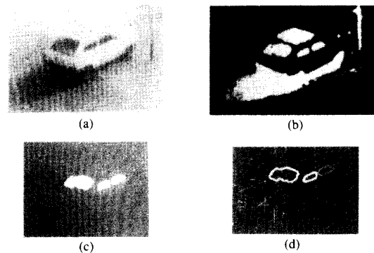
Fig. 1. (a) Original image of car. (b) After low-pass filter and binary threshold. (c) Line-labeled image. (d) After edge detection.
