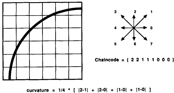
Fig. 3. Determination of curvature for contour segment within scan window.
