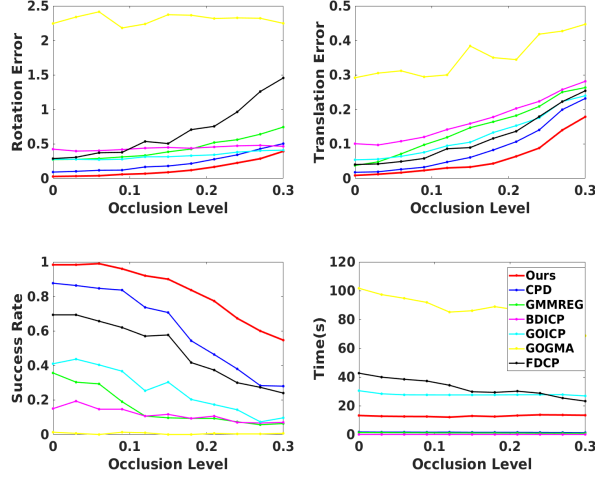
Figure 6: Occlusion Experiment
