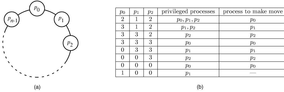
Fig. 1. (a) A ring network. (b) An example of a computation of the K -state algorithm ( n = 3 , K = 4 ).
