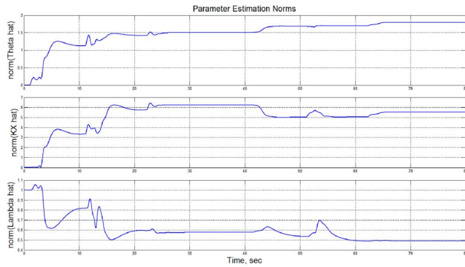
Fig. 4. Norms of estimated parameters in the presence of uncertainties.
