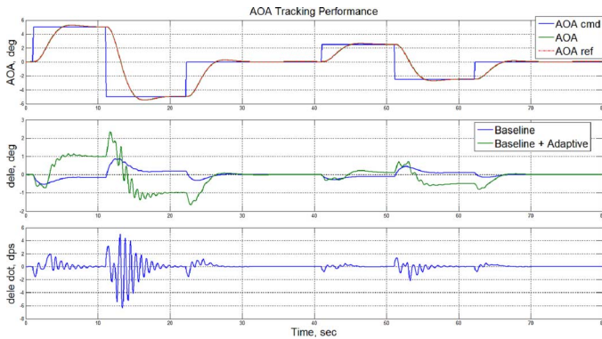
Fig. 5. (LQR + MRAC) response with uncertainties.
