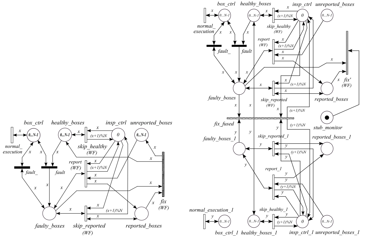
Figure 10. The COMMBBoxTECH ( n ) benchmark (left) and the corresponding verifier (right).
