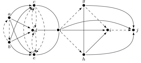
Figure 2. An example of generalised mutex order structure G .
