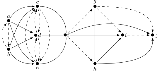
Figure 3. The closure of the structure S from Figure 1.
