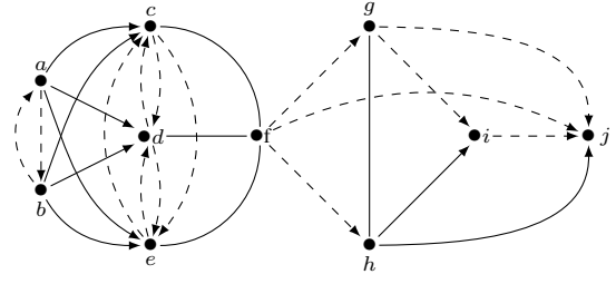
Figure 6. The integration of the structure S from Figure 1.
