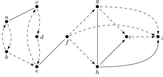
Figure 1. An example of reflexive order structure S .
