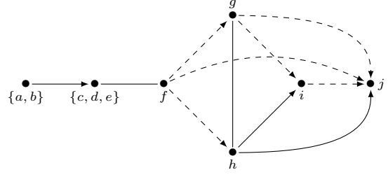
Figure 4. The folding of the structure S from Figure 1.
