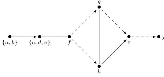
Figure 7. The folded reduction of the structure S from Figure 1.
