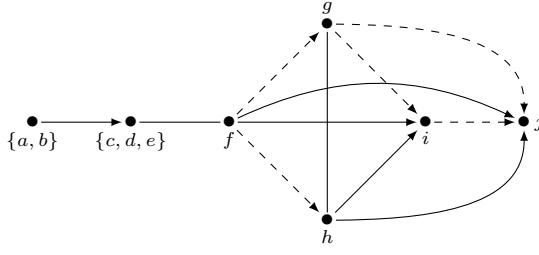
Figure 5. The folding of the structure S^c from Figure 3 equal to the closure of the structure S^f from Figure 4.
