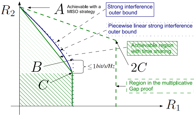
Fig. 5. A representation of the proof of Th.IV.1: the solid blue line is the outer bound in (1) and the dotted blue line the outer bound in (11); the green hatched region is the achievable region obtained with time sharing between the points A and C , while the green dotted line is the region in the converse of the multiplicative gap.
