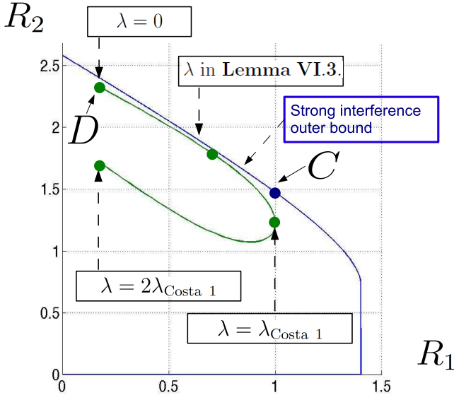
Fig. 7. A plot of the points C(\lambda) and D(\lambda) for \alpha = 0.5 , together with the “strong interference” bound for the real-valued G-CIFC with parameters P_1 = P_2 = 6 , b = \sqrt{2} and a = \sqrt{0.3} .
