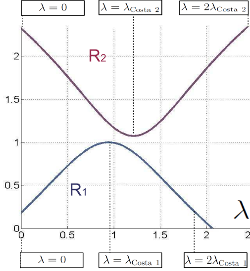
Fig. 3. The bound for R_1 in (7a) (bottom) and the bound for R_2 in (7b) (top) as a function of \lambda \in \mathbb{R} , for P_1 = P_2 = 6 , b = \sqrt{2} and a = \sqrt{0.3} and \alpha = 0.5 .
