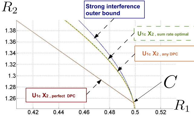
Fig. 7. A plot of the points C(\lambda) and D(\lambda) for \alpha = 0.5 , together with the “strong interference” bound for the real-valued G-CIFC with parameters P_1 = P_2 = 6 , b = \sqrt{2} and a = \sqrt{0.3} .
