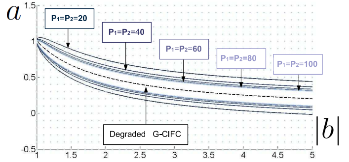
Fig. 6. The region where the condition in (12) is verified, for different values of P_1 = P_2 = P .
