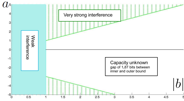
Fig. 2. A representation of the known capacity results for the real-valued G-CIFC with P_1 = P_2 and (a, |b|) \in [-5, 5] \times [0, 5] . The “weak interference” regime has solid light blue fill, while the “very strong interference” regime has dotted green lines.
