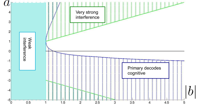
Fig. 4. A representation of the capacity result of Th.III.1 for a real-valued G-CIFC with P_1 = P_2 = 10 and (a, |b|) \in [-5, 5] \times [0, 5] . The “weak interference” regime has solid light blue fill, the “very strong interference” regime has dotted green lines, while the “primary decodes cognitive” region has dotted navy blue lines.
