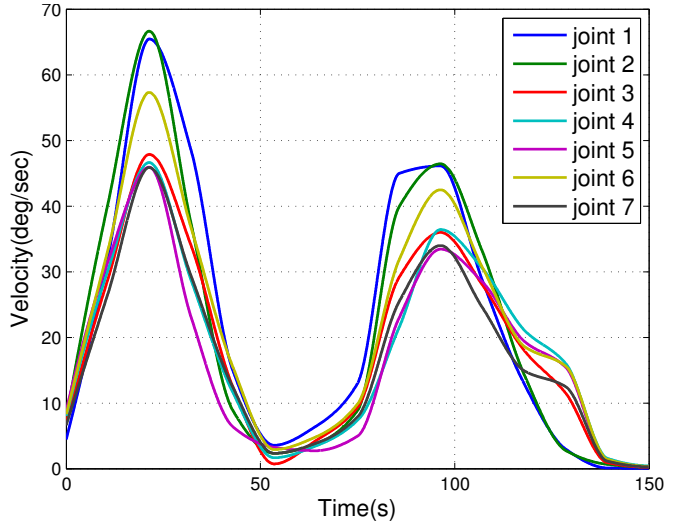
Figure 6. Joint velocities of left arm during picking the object.
