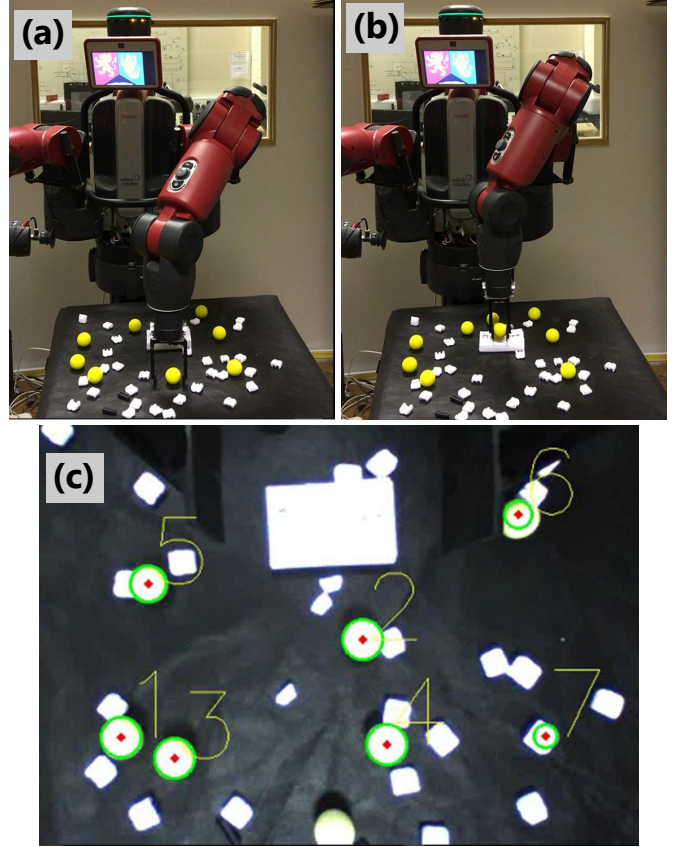
Figure 9. Single arm manipulation in cluttered scenes: (a) detecting the white box and yellow balls, (b) grasping a ball and placing it on the white box, (c) detected objects, automatically labeled in order of which object is to be grasped first. See supplementary video for clear illustration.
