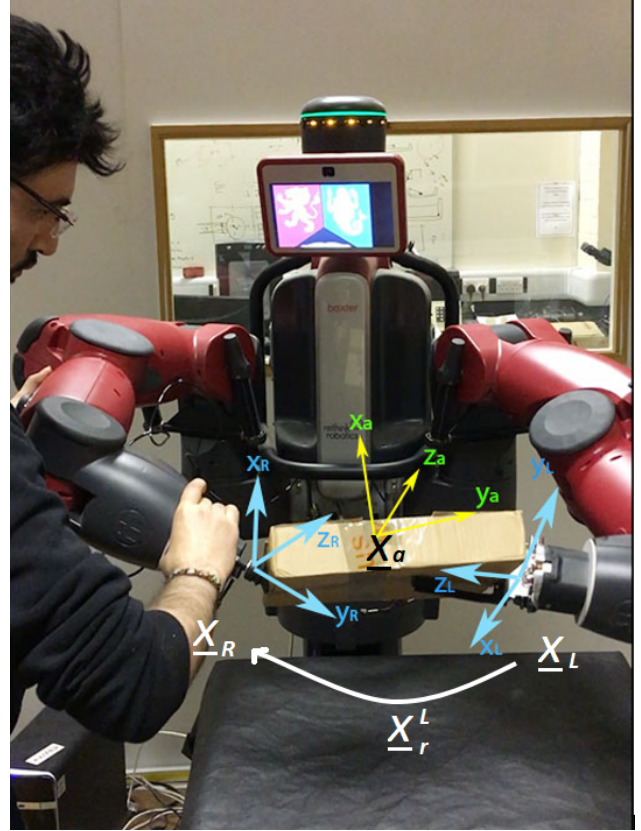
Figure 1. Master-slave manipulation based on task-space approach. The human moves the master arm in arbitrary ways. The slave arm is automatically controlled to maintain a constant transformation between the two end-effectors, thus preserving the bi-manual grasp on the box, regardless of the motions of the arms.
