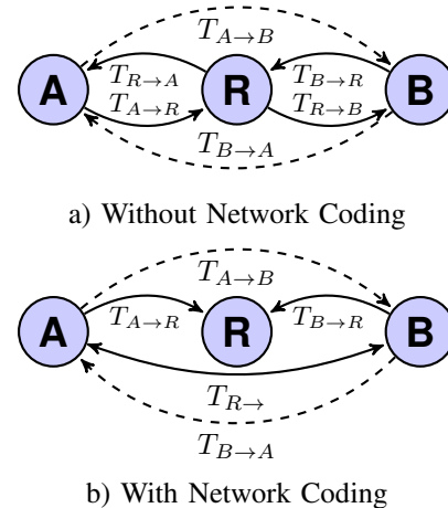
Fig. 1: Alice and Bob scenario with and without network coding. Solid line indicates the activity between the nodes, while the dashed line indicates the end-to-end throughput.
