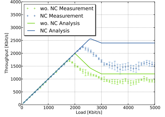
(a) Throughput Alice (A)
