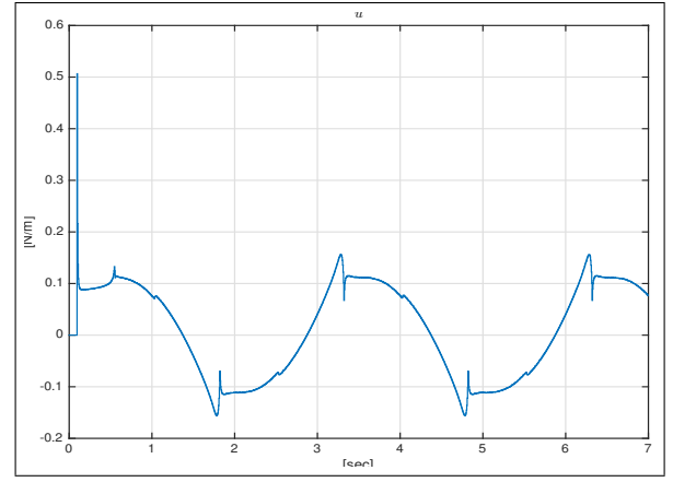
Fig. 5. Control law
