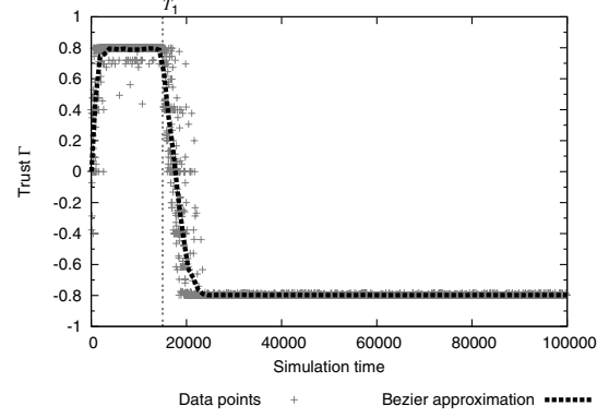
Figure 7. Fuzzy-Discrete
