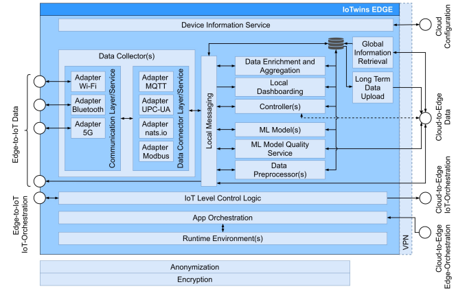
Figure 4: Edge Level Architecture
