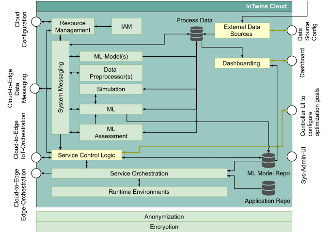
Figure 3: Cloud Level Architecture
