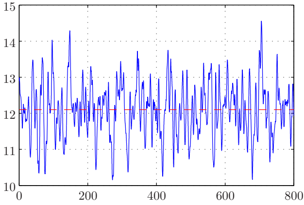
Fig. 10: Rotor rotational speed ( \omega_r ) (rpm)
