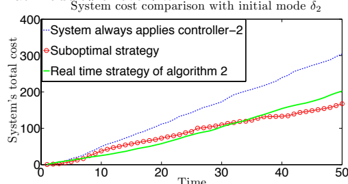
Fig. 4. Cost comparison of system applying different strategies at mode \delta_2 . Applying the suboptimal strategy provides the smallest cost, and the strategy of the real time algorithm is better than the one of a non-game approach.
