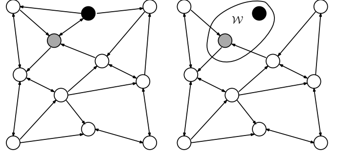
Fig. 3. On the left, the support graph \mathcal{G}_P of an irreducible stochastic matrix P . On the right, the support graph \mathcal{G}_{\tilde{P}} of a perturbed matrix \tilde{P} obtained as in Example 3, with node u colored in black and the rest of the perturbation set \mathcal{W} (consisting of the in-neighbors of u in \mathcal{G}_P ) colored in grey.
