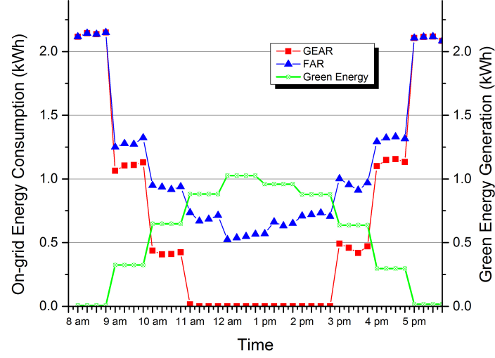
Fig. 6. On-grid energy consumption at different time
