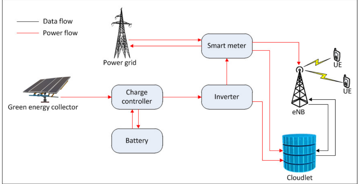
Fig. 2. The power supply system of the cloudlet.
