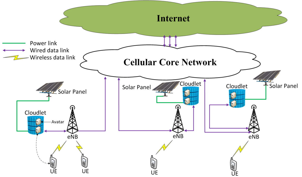
Fig. 1. Green cloudlet network architecture.
