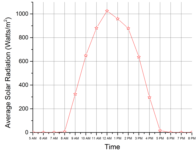
Fig. 5. Average solar radiation generated at different time
