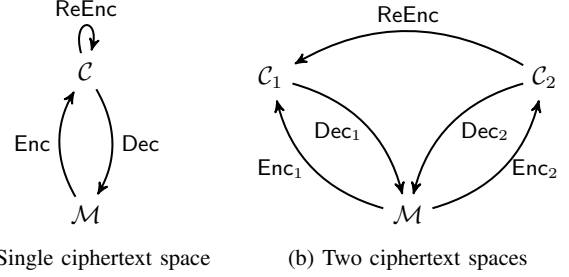
(a) Single ciphertext space (b) Two ciphertext spaces Fig. 1: Transformations between plaintext and ciphertext spaces
