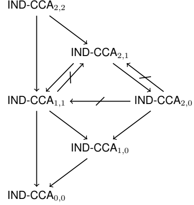
Fig. 5: Relations among security notions for multihop PRE
