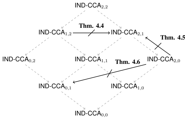
Fig. 3: Separations among notions of security.
