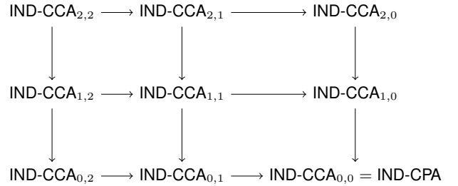
Fig. 2: Implications among security notions for PRE
