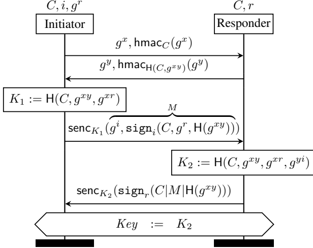
Figure 1: Secure Scuttlebutt’s ‘Secret Handshake’
