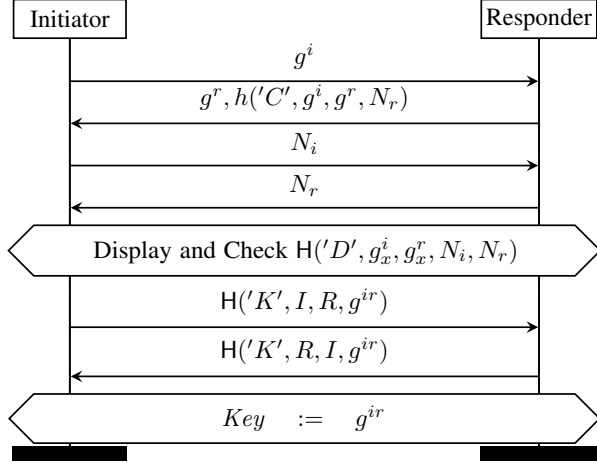
Figure 2: Bluetooth's Simple Secure Pairing Handshake
