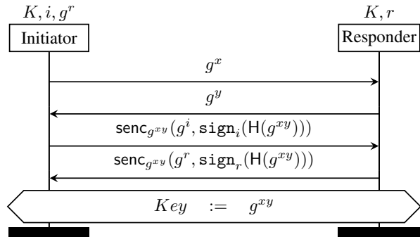
Figure 3: Tendermint's Handshake
