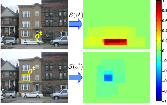
Figure 3: Classifier score force \mathcal{S} . (Left) Image and observation o^t . (Right) Belief map produced by \mathcal{S} . Colours correspond to belief values.
