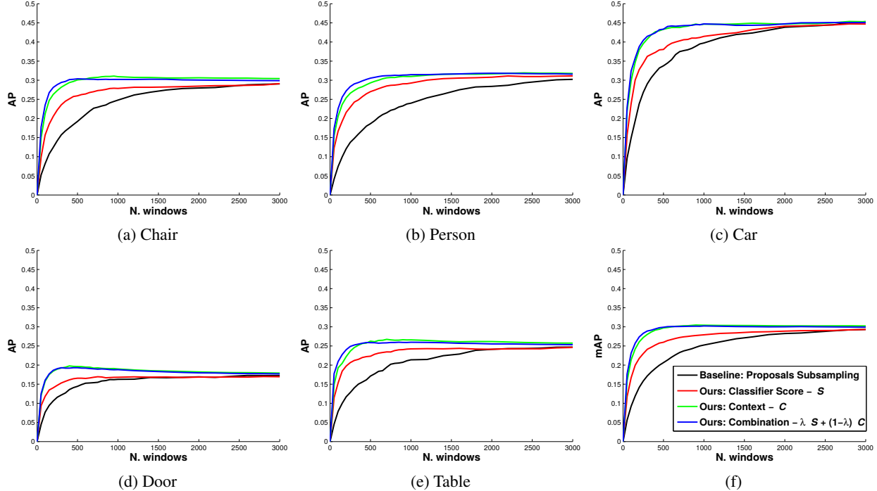
Figure 7: Results for SUN2012. Results for the baseline Proposals Subsampling and our method on SUN2012, using each force S , C alone and in combination. The x-axis shows the number of evaluated windows. The y-axis in (a-e) shows the AP of each class, while in (f) it shows the mean AP over all classes (mAP).
