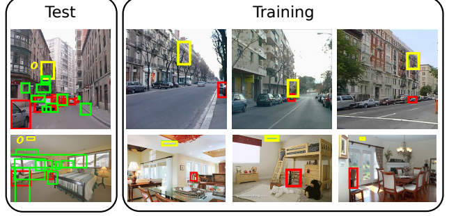
Figure 6: RF examples. (Test) Example image and observation o for classes car (top) and chair (bottom). Windows displaced by the displacement vectors regressed by the RF are in green, whereas ground-truth objects are in red. (Training) Training samples (yellow) in leaves reached by o when input into our RF and associated ground-truth objects (red).
