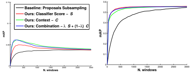
Figure 8: (Left) Results on SUN2012 using the UvA detector [49]. (Right) Results on PASCAL VOC10 using R-CNN.
