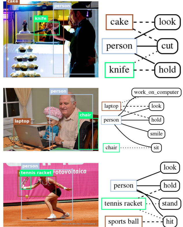
Figure 3. Example VSP graphs generated by our method. Solid, dashed, and dotted lines represent subject, object, and instrument.
